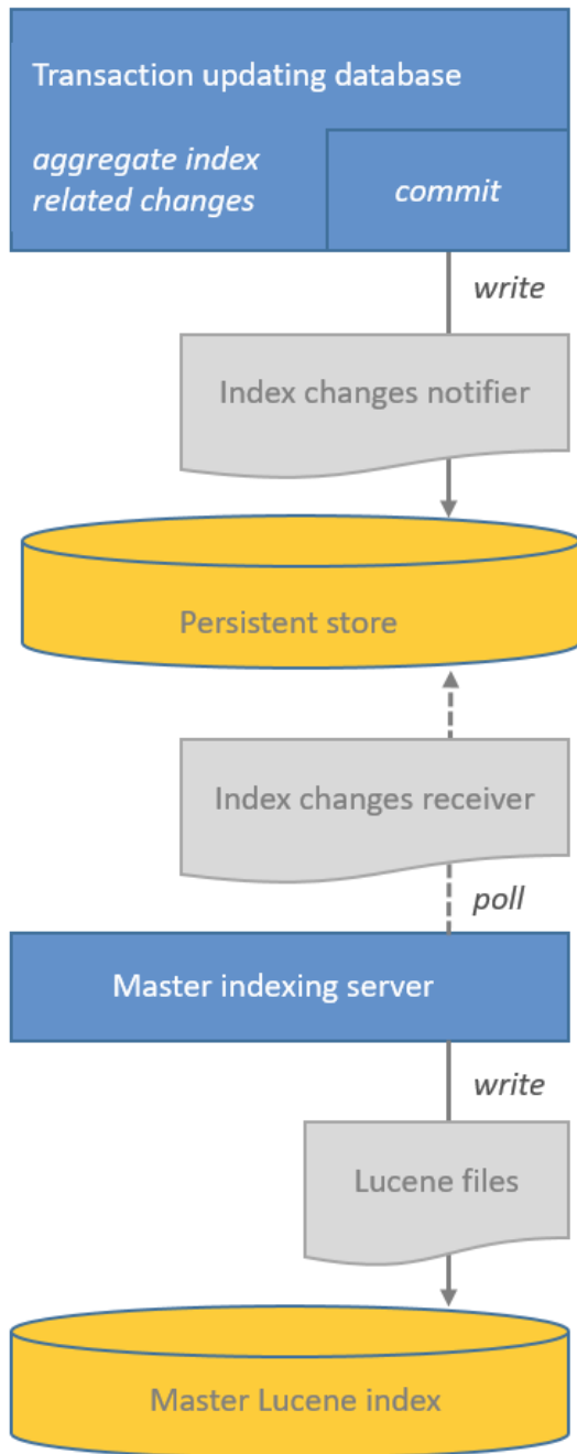
Figure 375: Indexer architecture in a single-server environment
