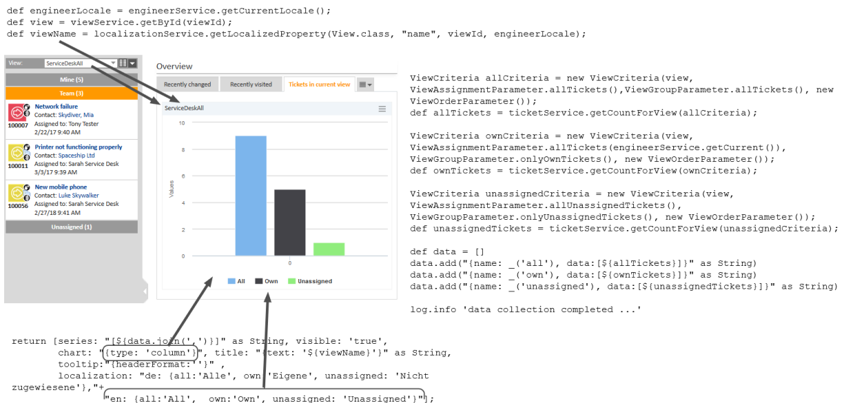
Figure 302: Chart widget example with script code
