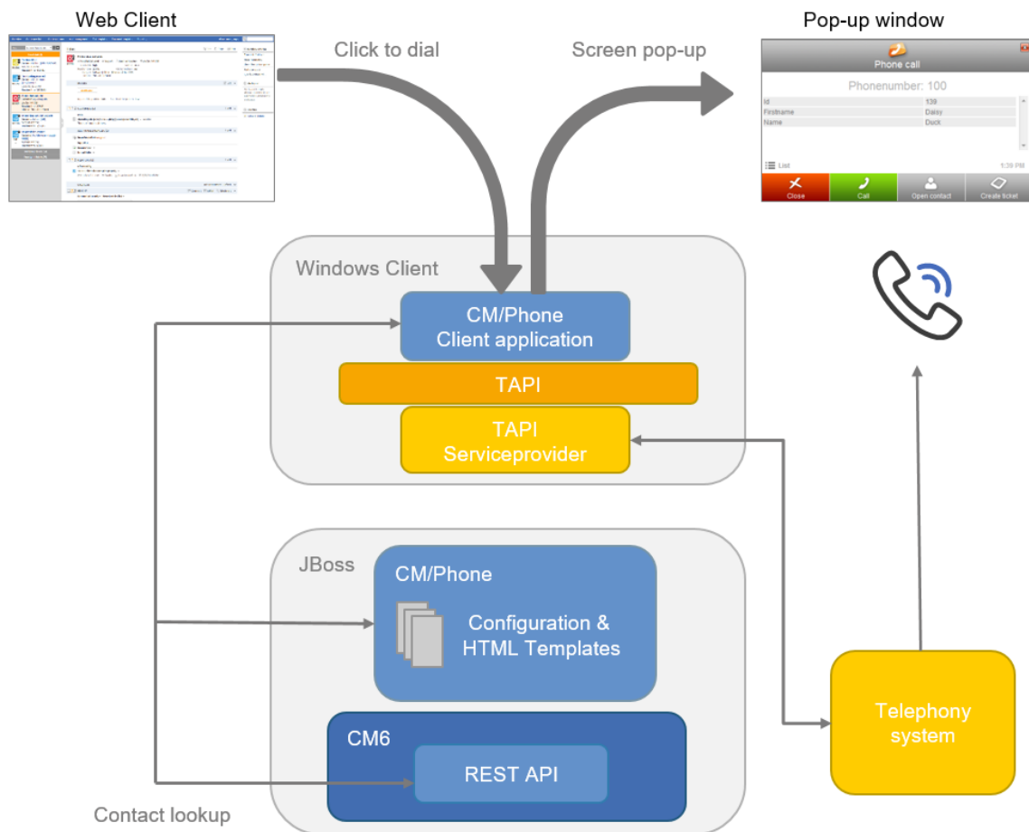
Figure 641: ConSol CM/Phone - Basic principle
