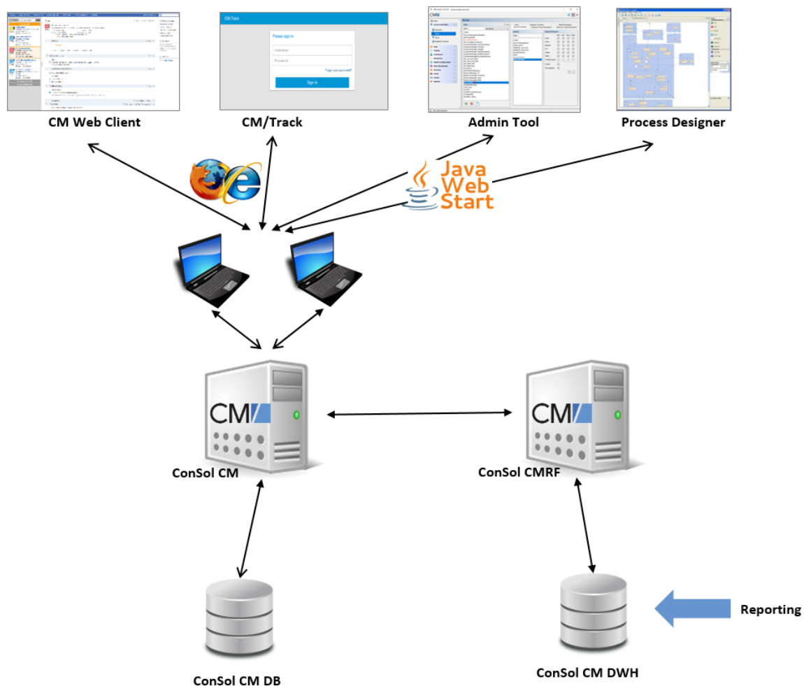
Figure 534: ConSol CM - Infrastructure with CMRF and DWH (2 servers)
