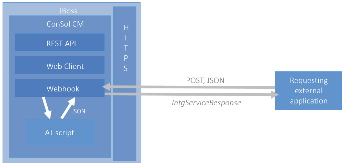
Figure 529: Basic principle of the ConSol CM Webhooks
