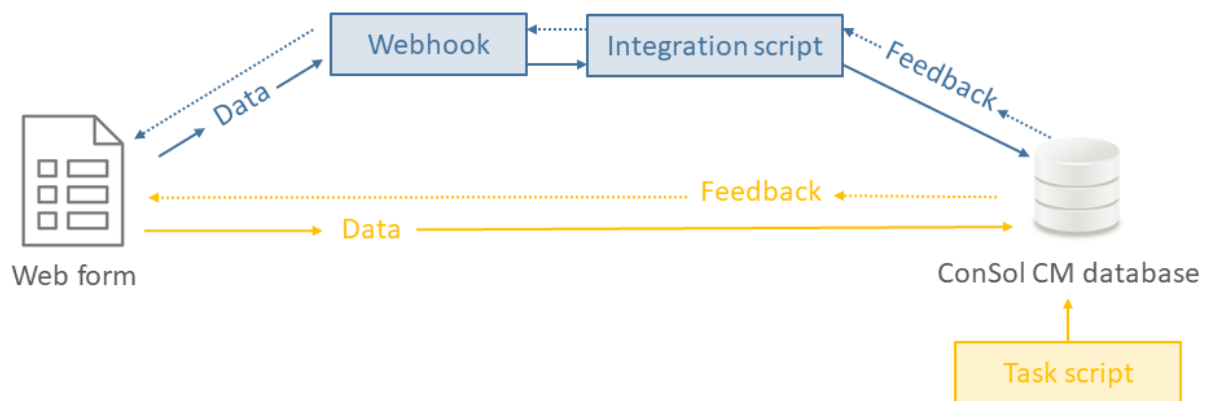
Figure 632: Data processing for web forms
