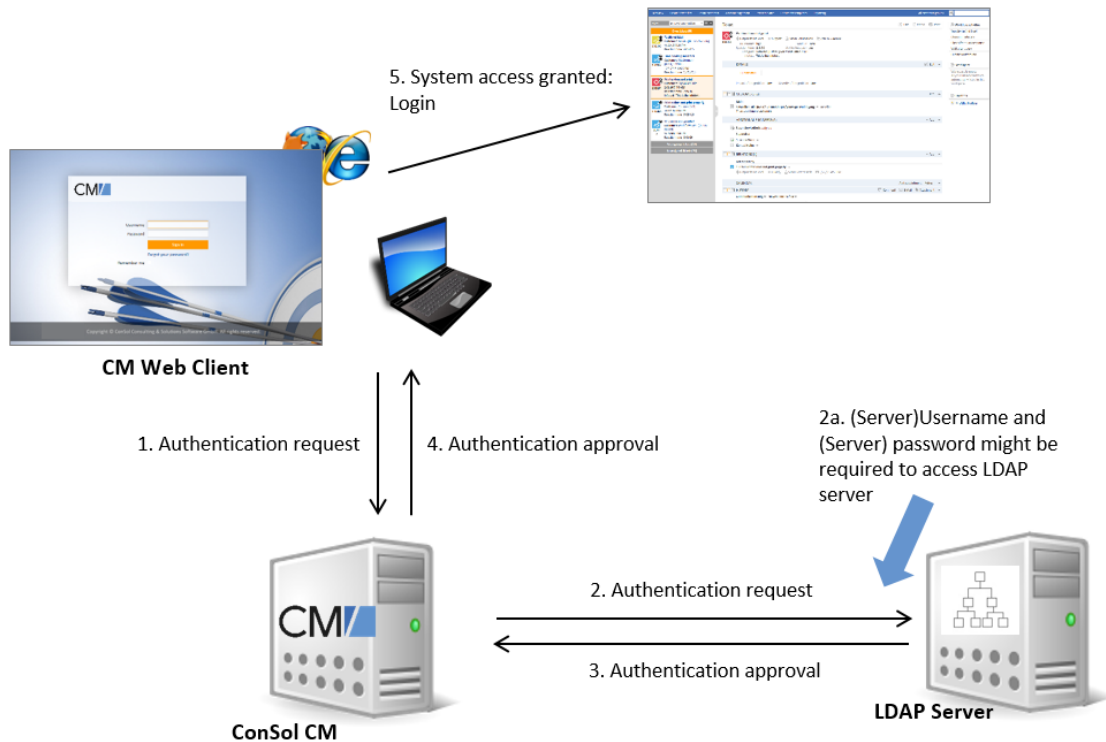
Figure 521: ConSol CM - LDAP authentication process
