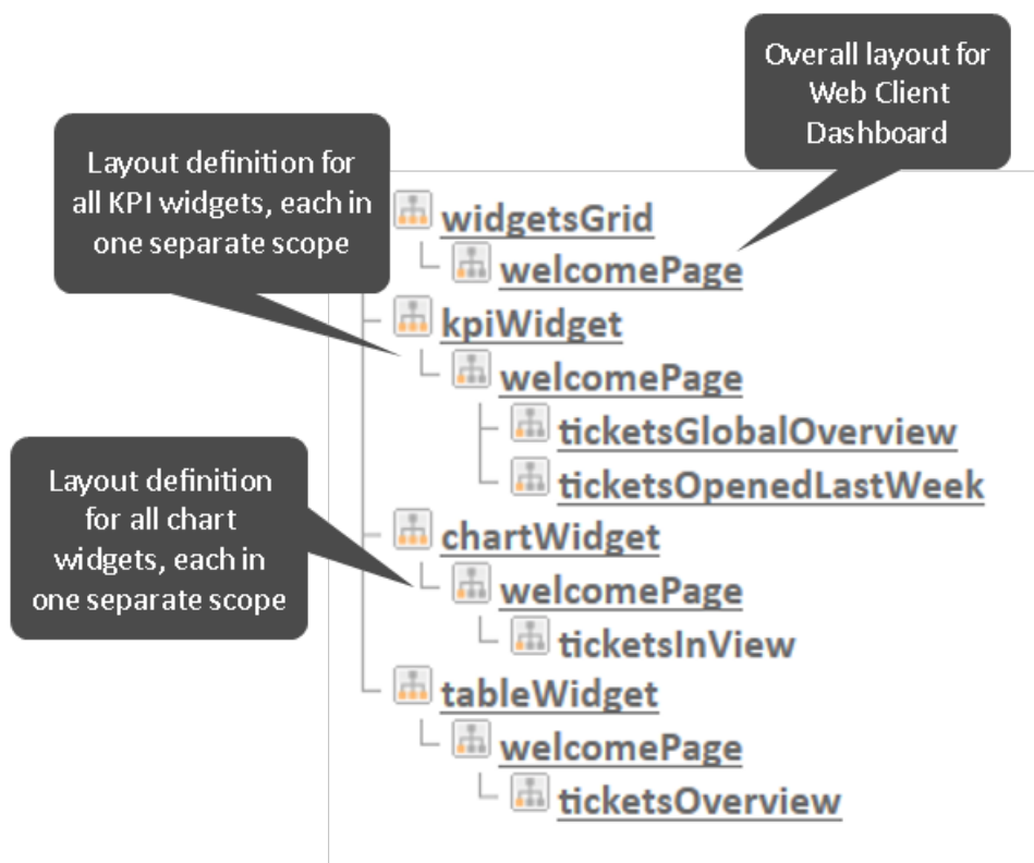
Figure 286: ConSol CM Web Client - Page customization subtrees for Web Client dashboard layout
