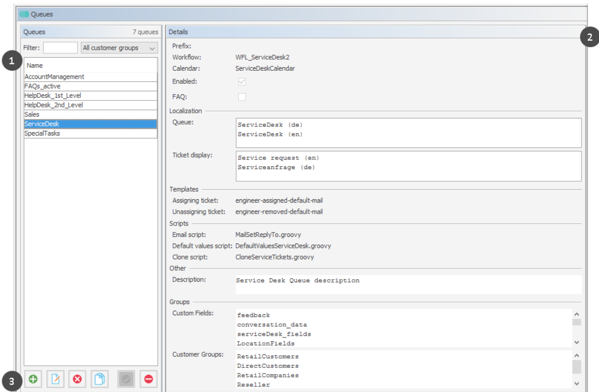
Figure 170: ConSol CM Admin Tool - Global Configuration, Queues: Queue administration
