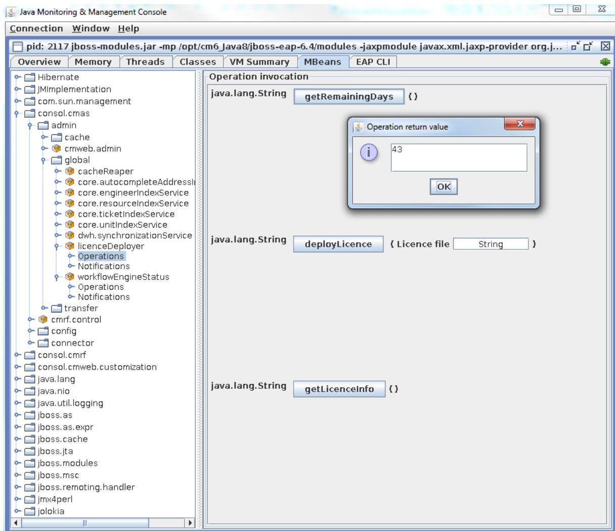
Figure 427: Retrieving the remaining days of a CM license using the JConsole
