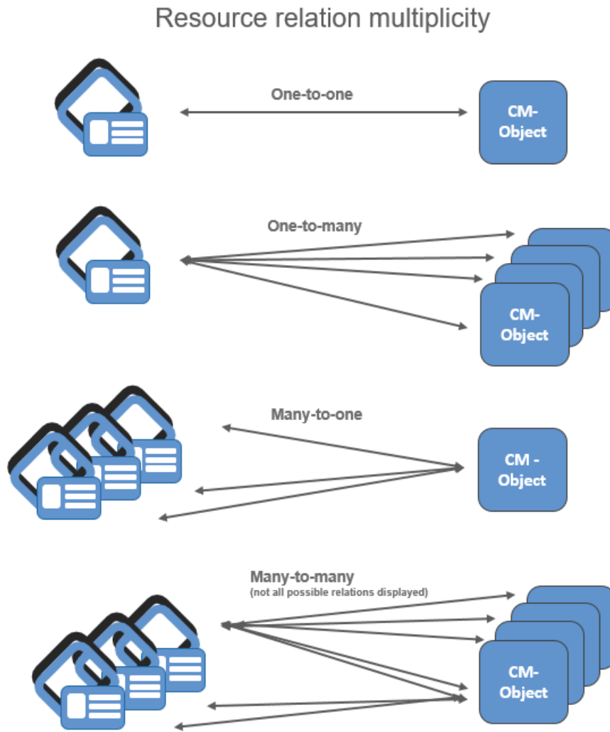
Figure 545: ConSol CM resource relation multiplicity
