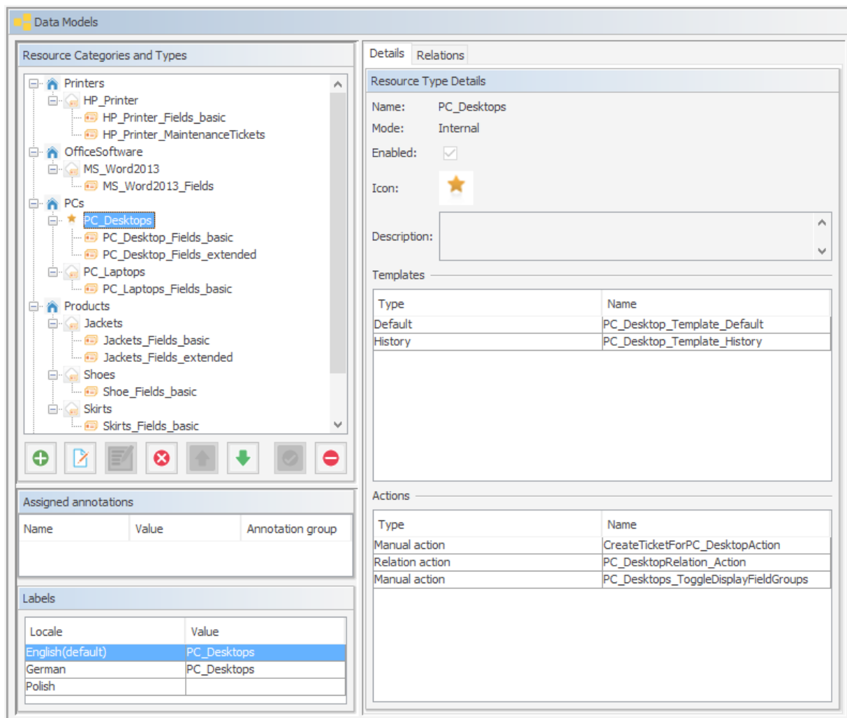
Figure 502: ConSol CM Admin Tool - Resources, Data Models: Simple Resource Pool configuration
