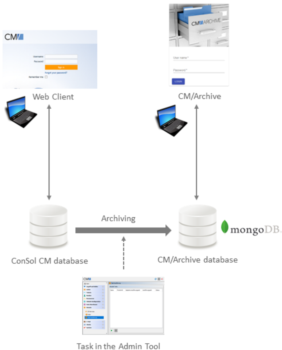
Figure 598: Architecture of ConSol CM with CM/Archive
