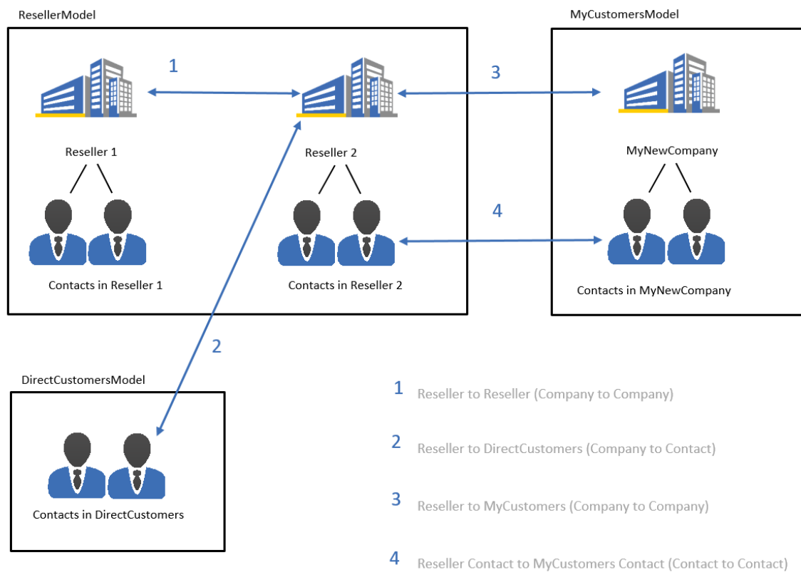
Figure 136: ConSol CM customer data model - Examples of customer relations
