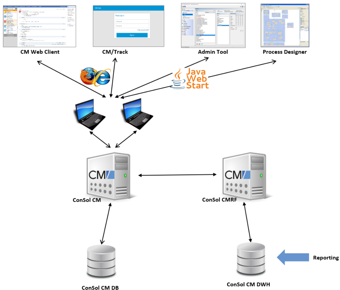
Figure 344: ConSol CM - System architecture with DWH and CMRF (2 servers)
