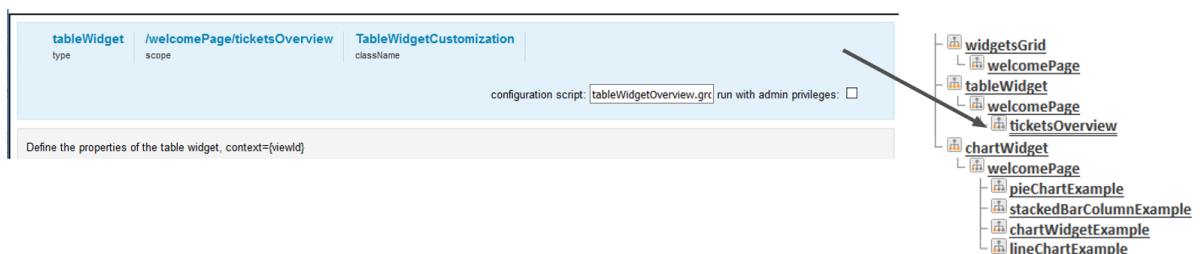
Figure 305: ConSol CM Web Client - Configuration of example table widget
