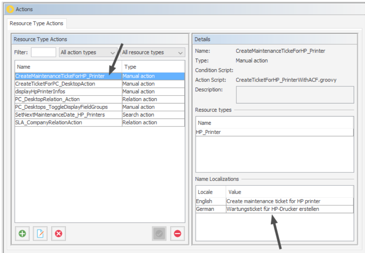
Figure 517: ConSol CM Admin Tool - Resources, Actions: Definition of a resource action
