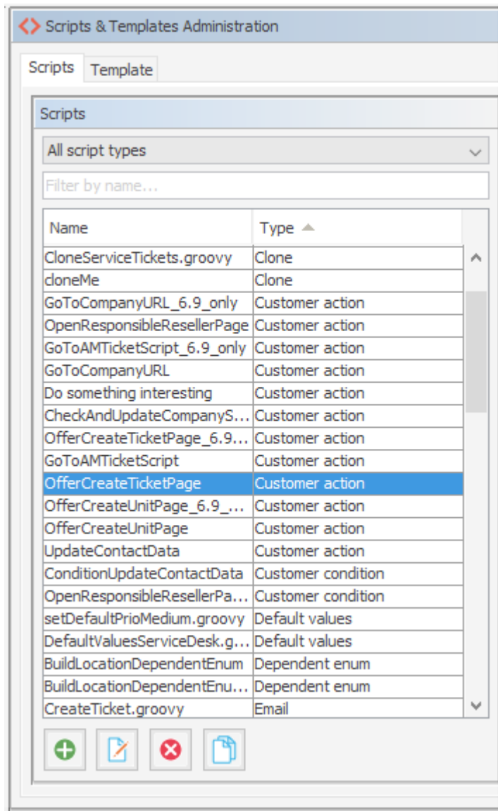
Figure 141: ConSol CM Admin Tool - System, Scripts and Templates: Scripts for customer actions
