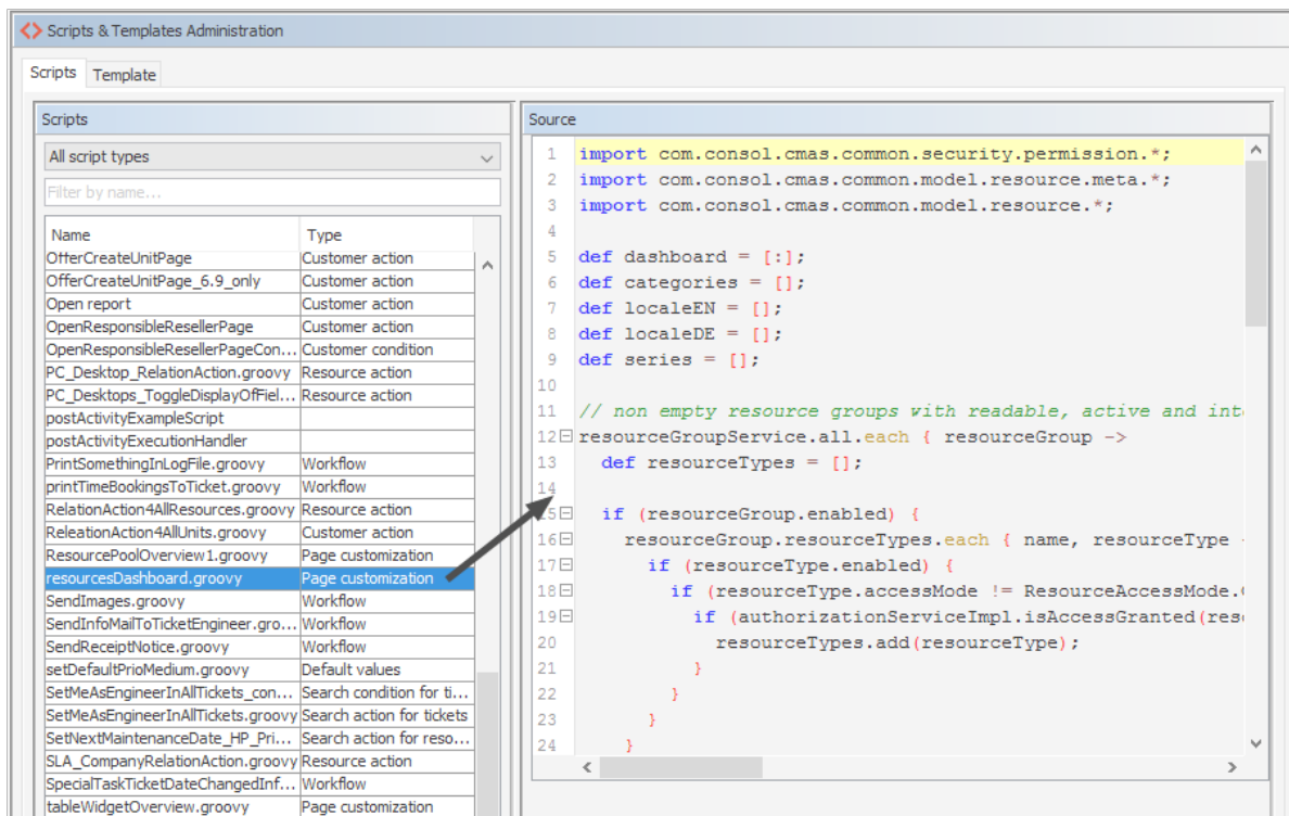
Figure 570: ConSol CM Admin Tool - System, Scripts and Templates: Admin Tool script for a widget of the Resource Pool Dashboard
