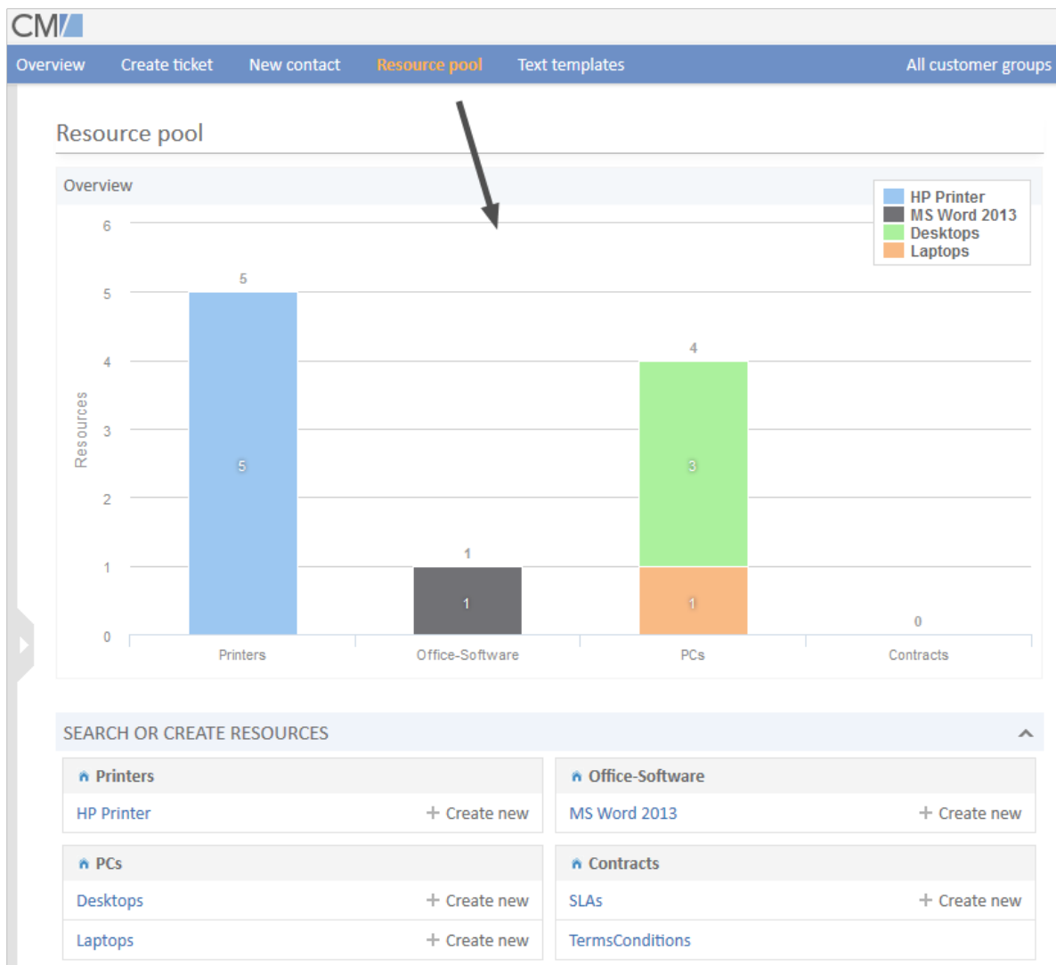
Figure 505: ConSol CM Web Client - Resource Pool Dashboard
