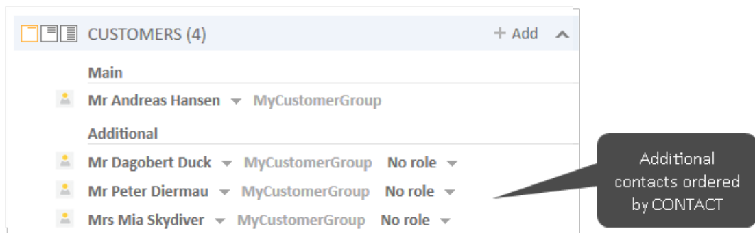
Figure 245: ConSol CM Web Client - Page customization for sort order of additional customers (3)
