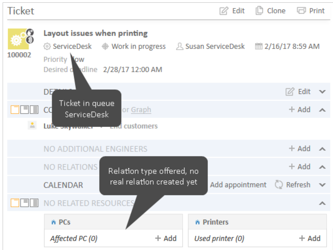
Figure 513: ConSol CM Web Client - Ticket where a relation to a PC can be created
