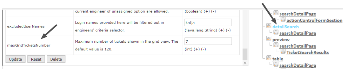
Figure 261: ConSol CM Web Client - Using page customization to adapt maximum number of tickets shown in grid
