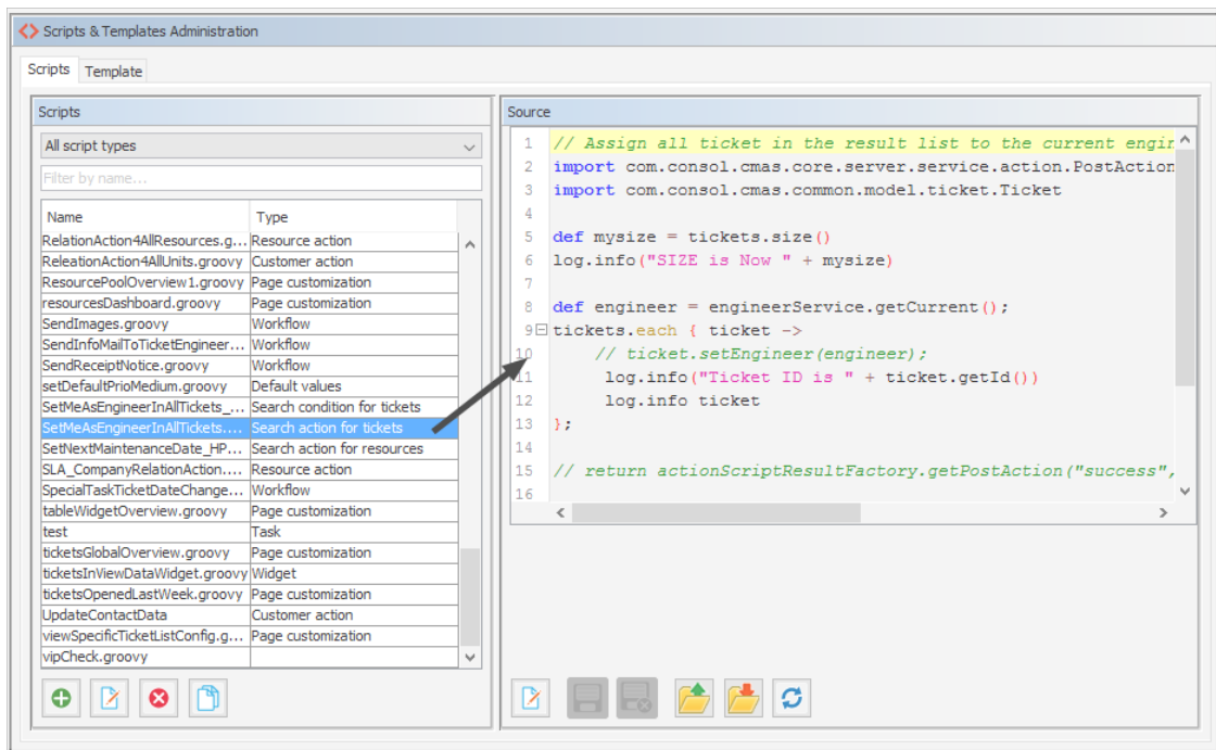
Figure 369: ConSol CM Admin Tool - System, Scripts and Templates: Script for a search action for tickets
