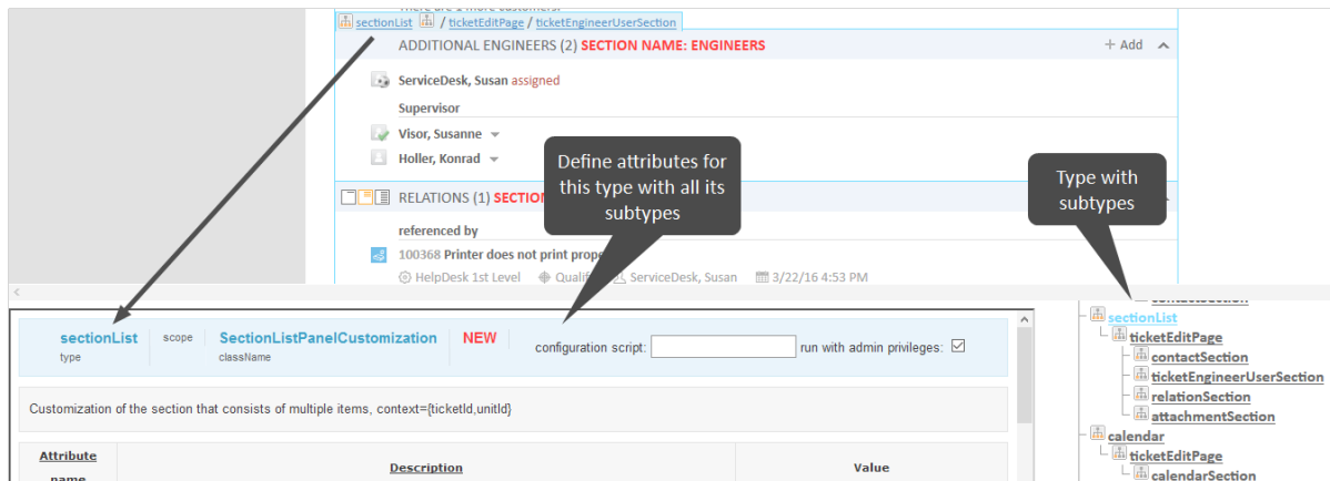
Figure 200: Selecting the level for the Page Customization, here: type.
