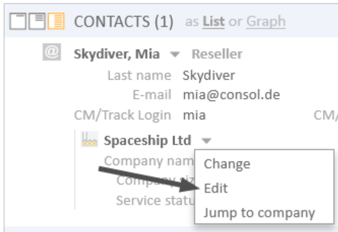
Figure 246: ConSol CM Web Client - Visibility of company Edit link ( companyEditLinkVisible = true )
