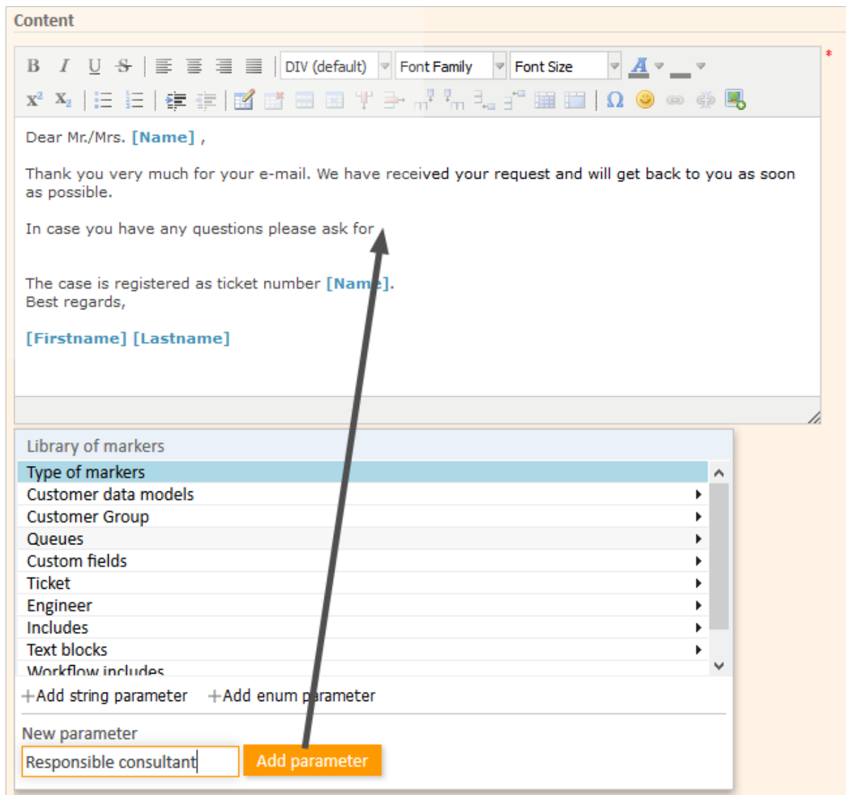
Figure 433: ConSol CM Web Client - Text Template Manager: Add string parameter in Library of markers
