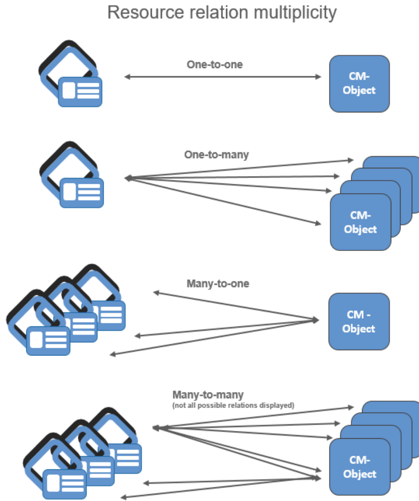
Figure 538: ConSol CM resource relation multiplicity
