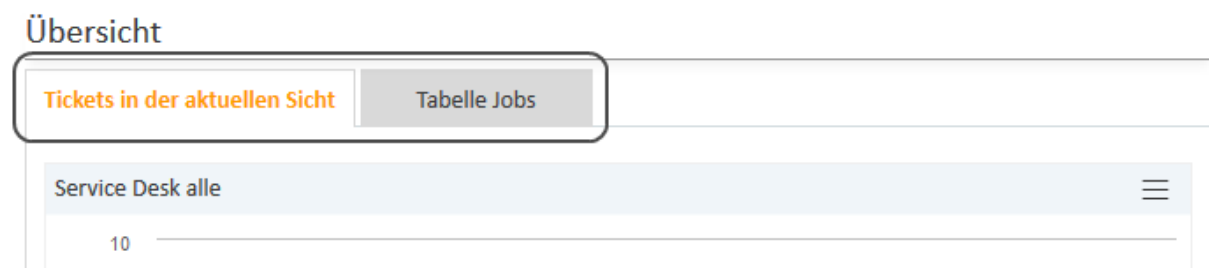
Figure 284: Using localized headers (in the given example en and de, displayed: de)
