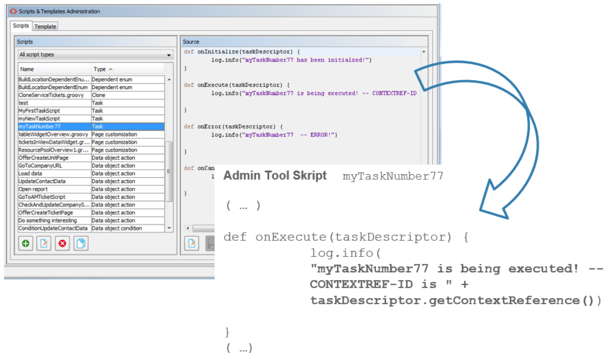
Figure 385: ConSol CM Admin Tool - System, Scripts and Templates: Admin Tool script for a TEF task
