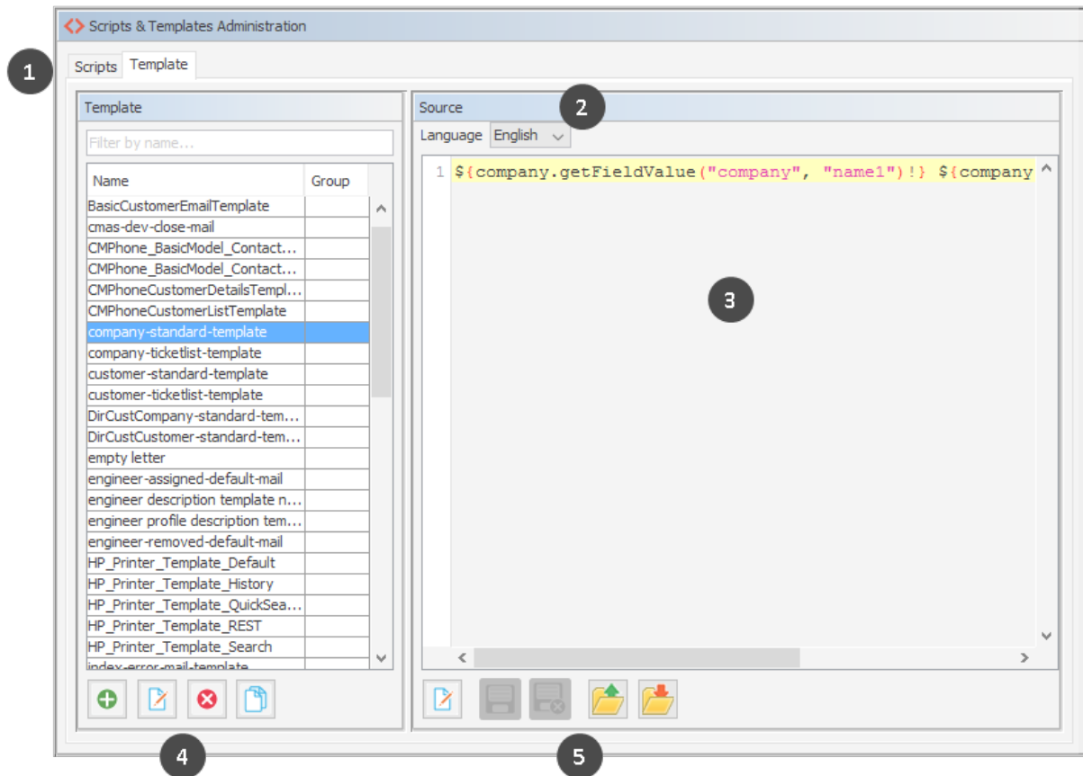
Figure 413: ConSol CM Admin Tool - System, Scripts and Templates: Template editor
