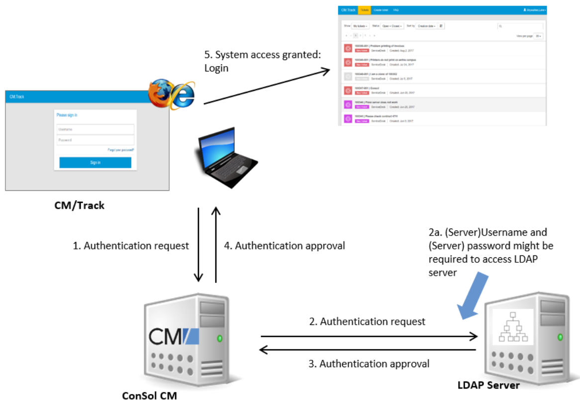
Figure 481: ConSol CM - LDAP authentication process for CM/Track
