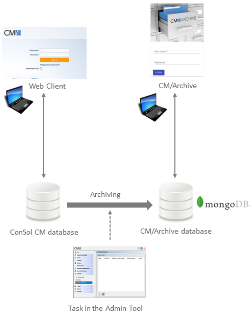
Figure 591: Architecture of ConSol CM with CM/Archive
