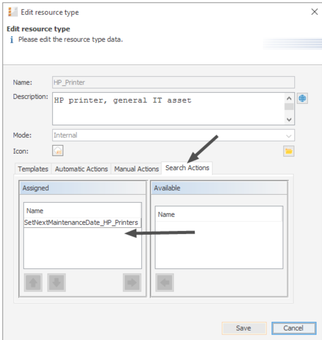
Figure 366: ConSol CM Admin Tool - Resources, Actions: Assigning a search action to a resource type
