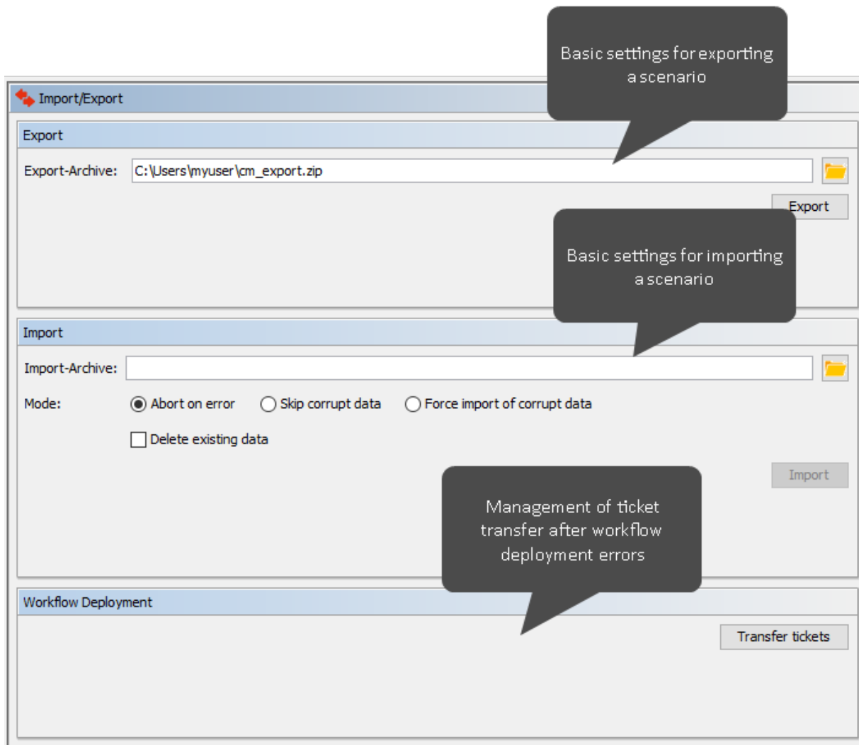
Figure 419: ConSol CM Admin Tool - System, Import/Export
