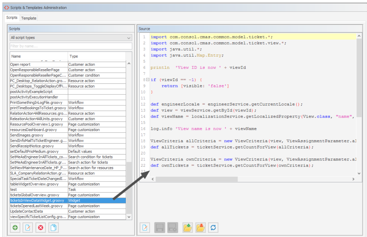
Figure 287: ConSol CM Admin Tool - Admin Tool script for a widget of the Web Client dashboard
