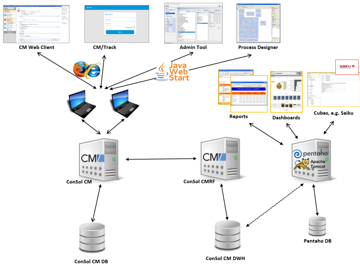
Figure 490: ConSol CM - Reporting infrastructure (2 servers)
