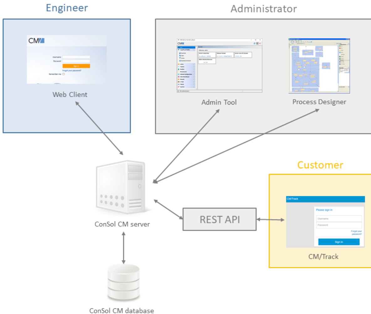
Figure 565: ConSol CM system architecture with CM/Track
