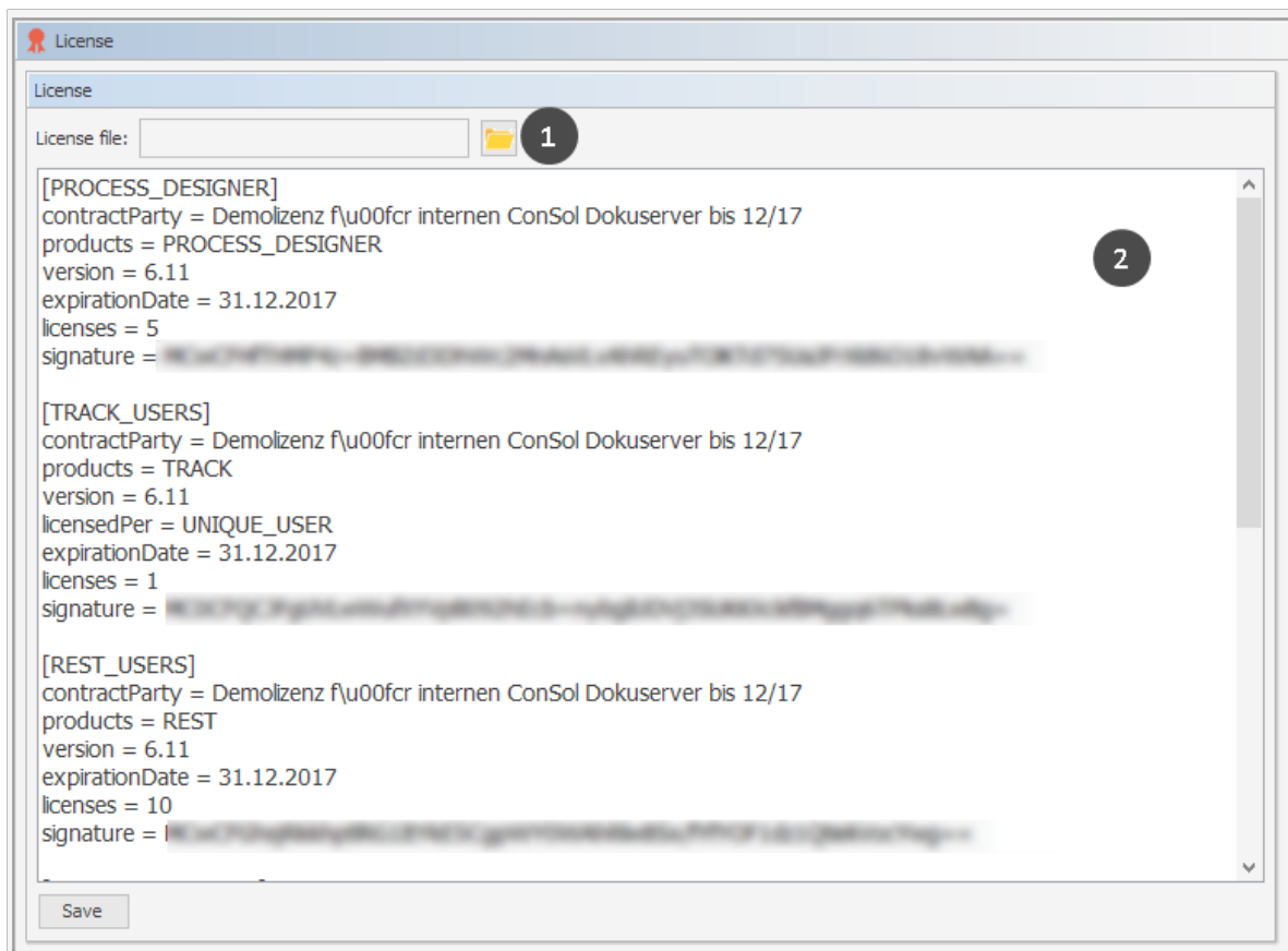
Figure 420: ConSol CM Admin Tool - System, License
