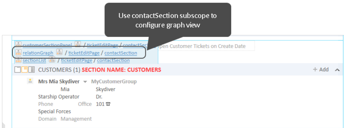
Figure 304: ConSol CM Web Client - Selection of page customization scope for relationGraph in contactSection
