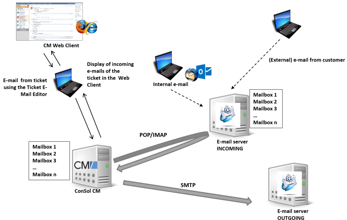
Figure 492: ConSol CM - Mail server interactions
