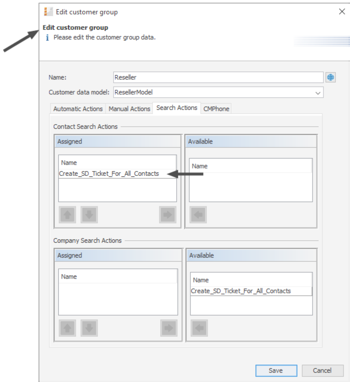
Figure 371: ConSol CM Admin Tool - Customers, Customer Groups: Assigning a search action to a contact object within a customer group
