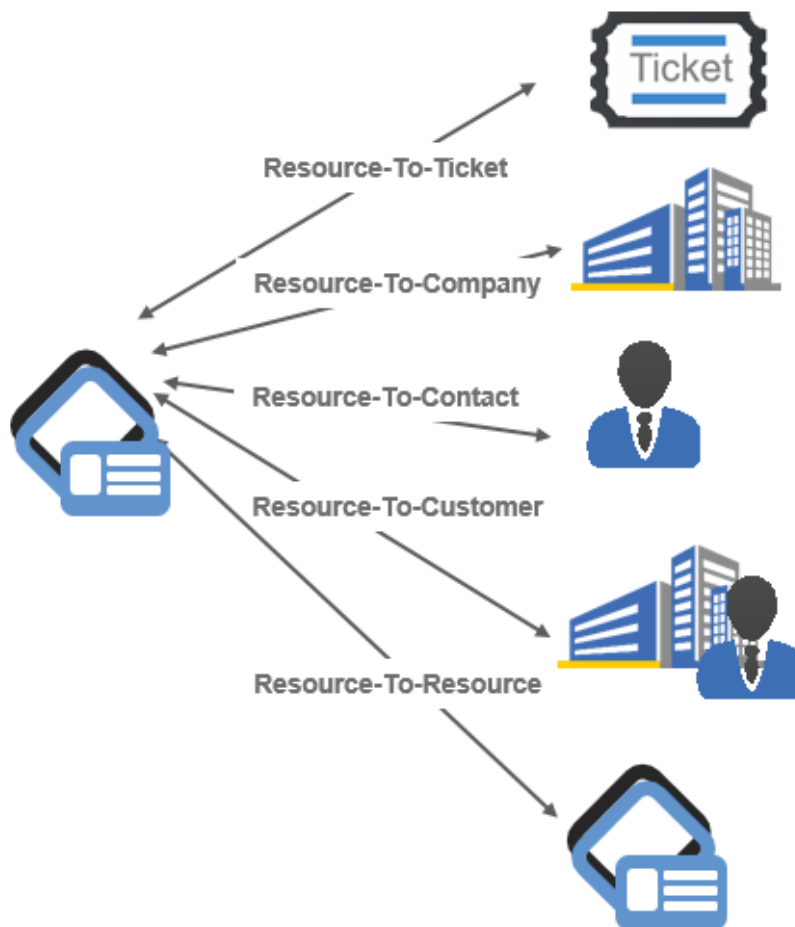
Figure 537: ConSol CM resource relation types
