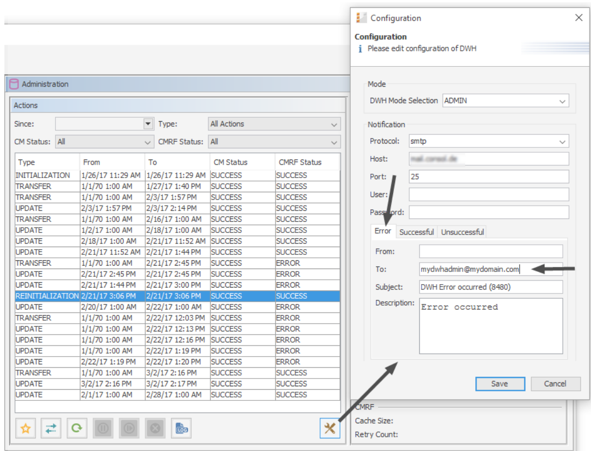
Figure 563: ConSol CM Admin Tool - Data Warehouse, Administration: Notification address for DWH errors
