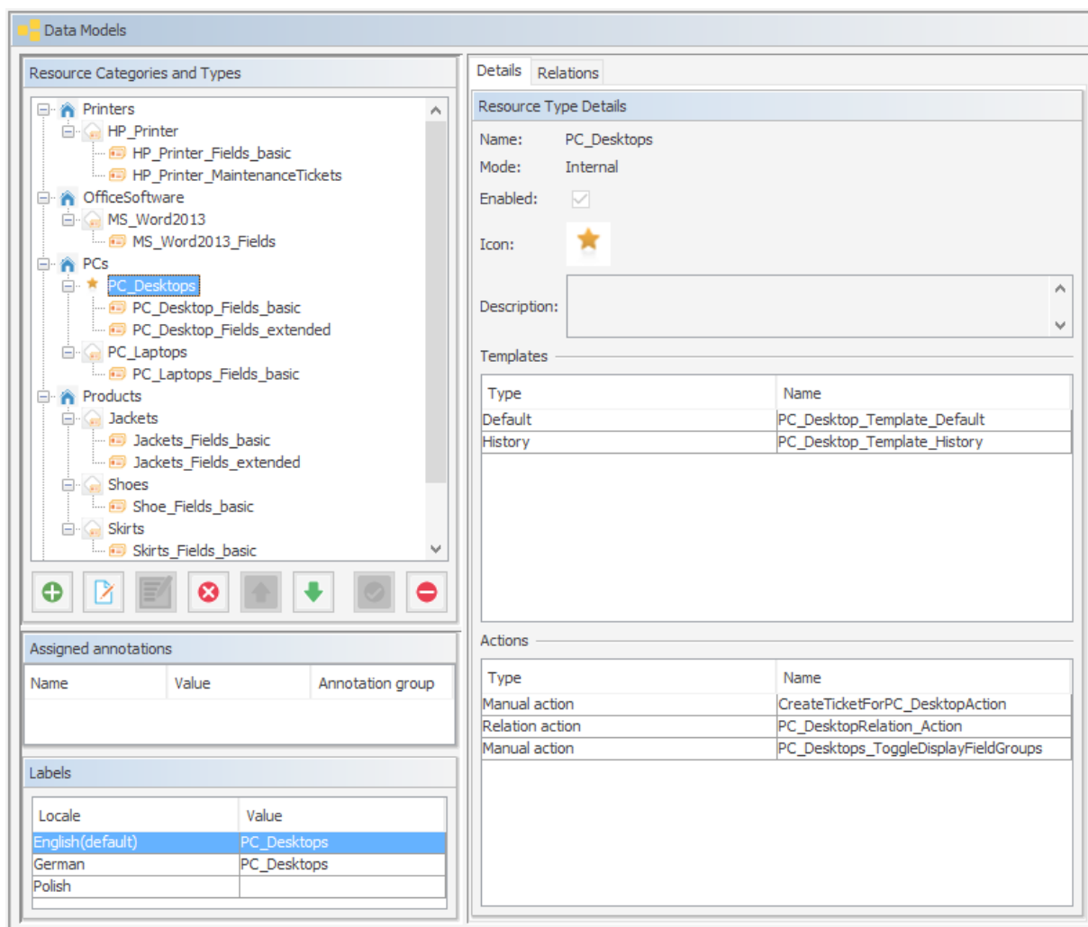
Figure 453: ConSol CM Admin Tool - Resources, Data Models: Simple Resource Pool configuration
