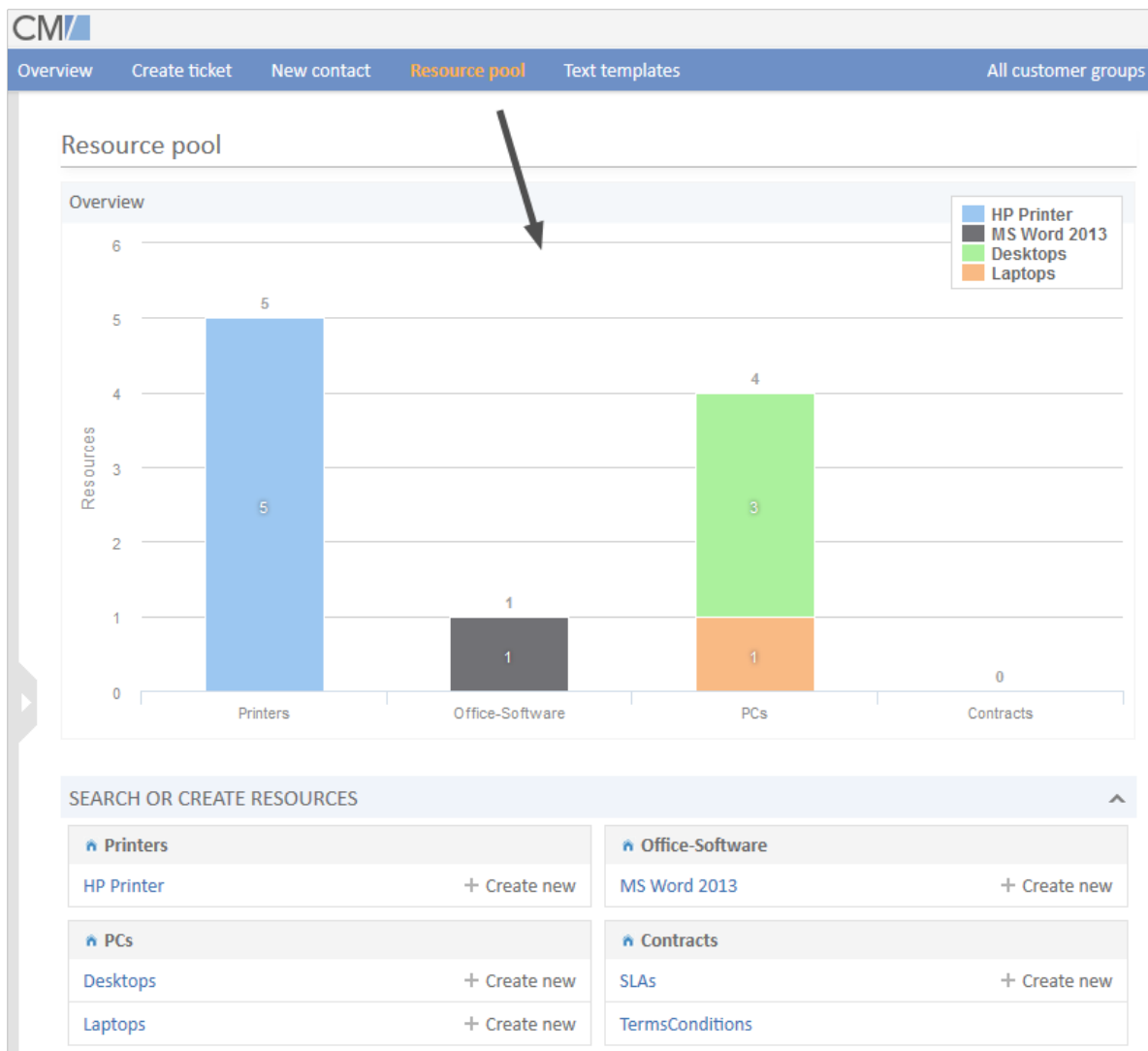
Figure 456: ConSol CM Web Client - Resource Pool Dashboard
