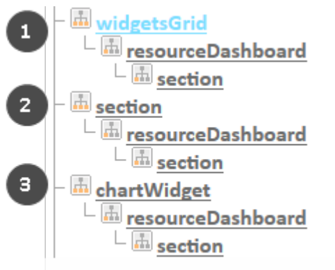
Figure 518: ConSol CM Web Client - Page Customization subtree for Resource Pool Dashboard configuration
