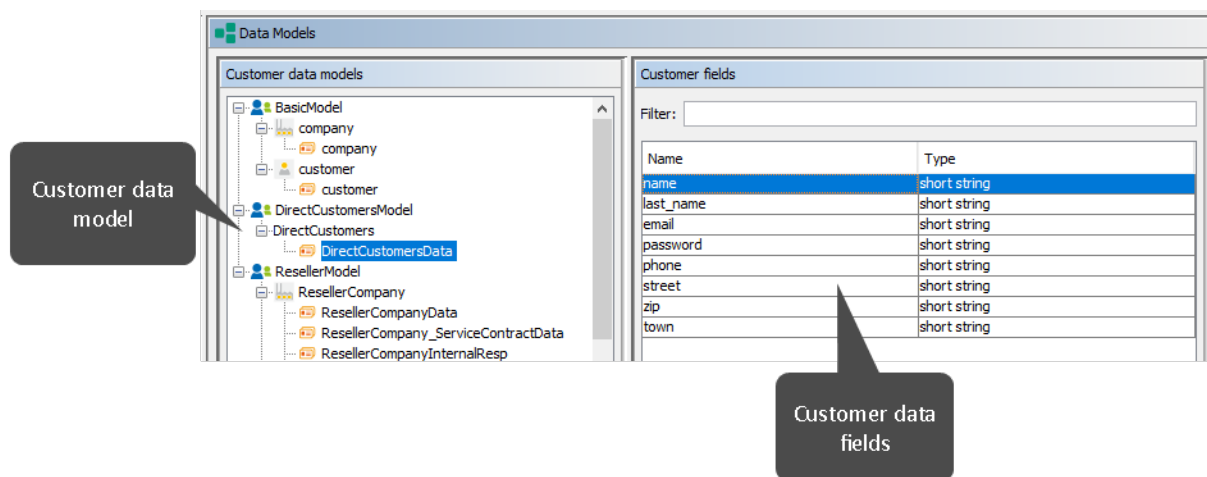
Figure 547: ConSol CM Admin Tool - Customers, Data Models: Example data fields
