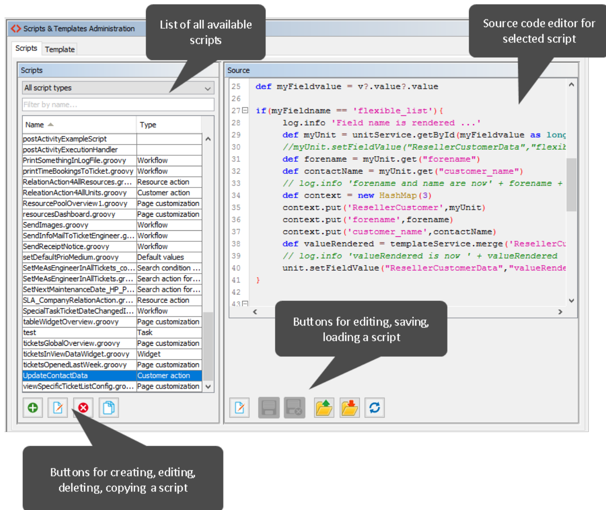
Figure 397: ConSol CM Admin Tool - System, Scripts and Templates
