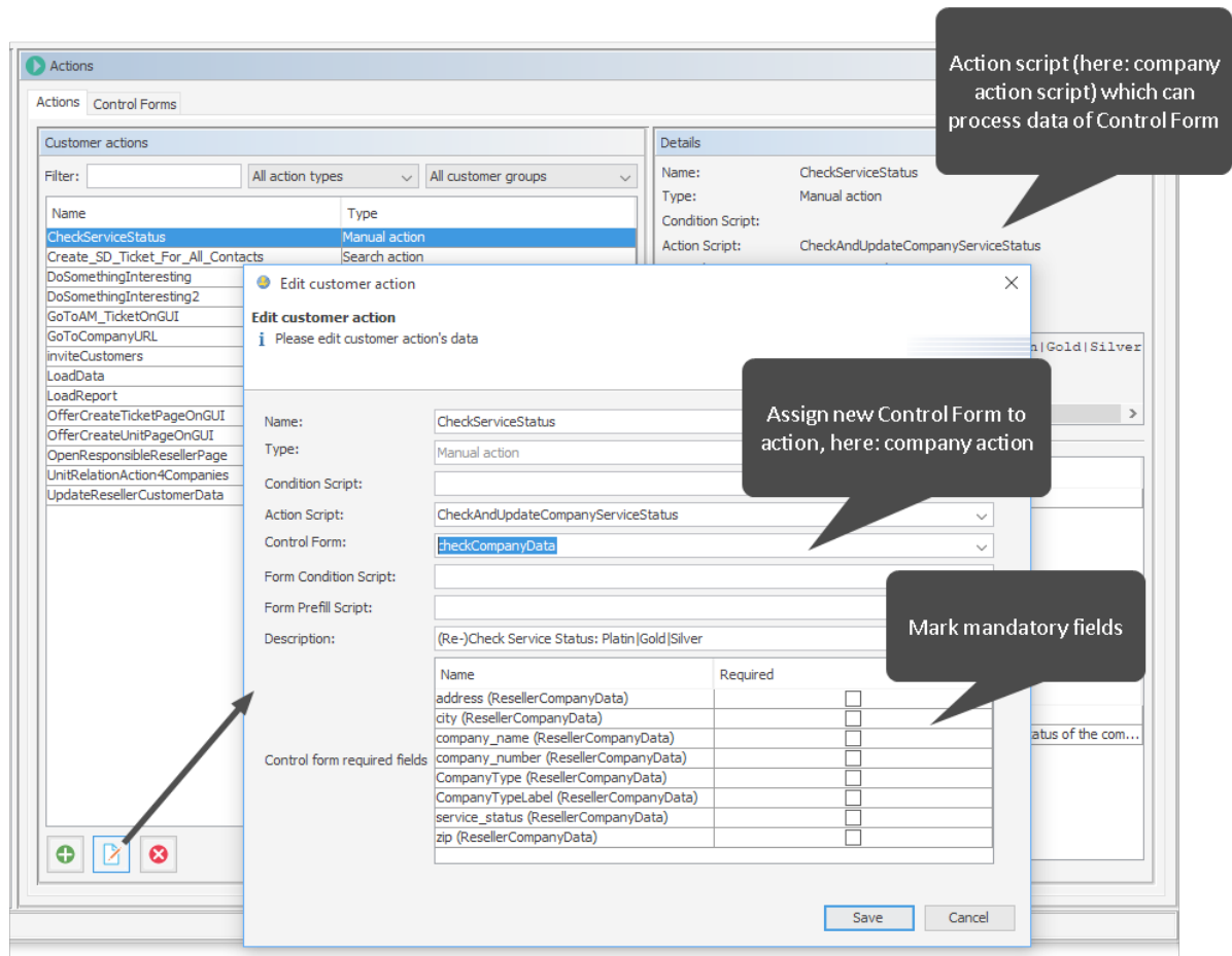
Figure 384: ConSol CM Admin Tool - Customers, Actions: Assigning a new Control Form to a company action
