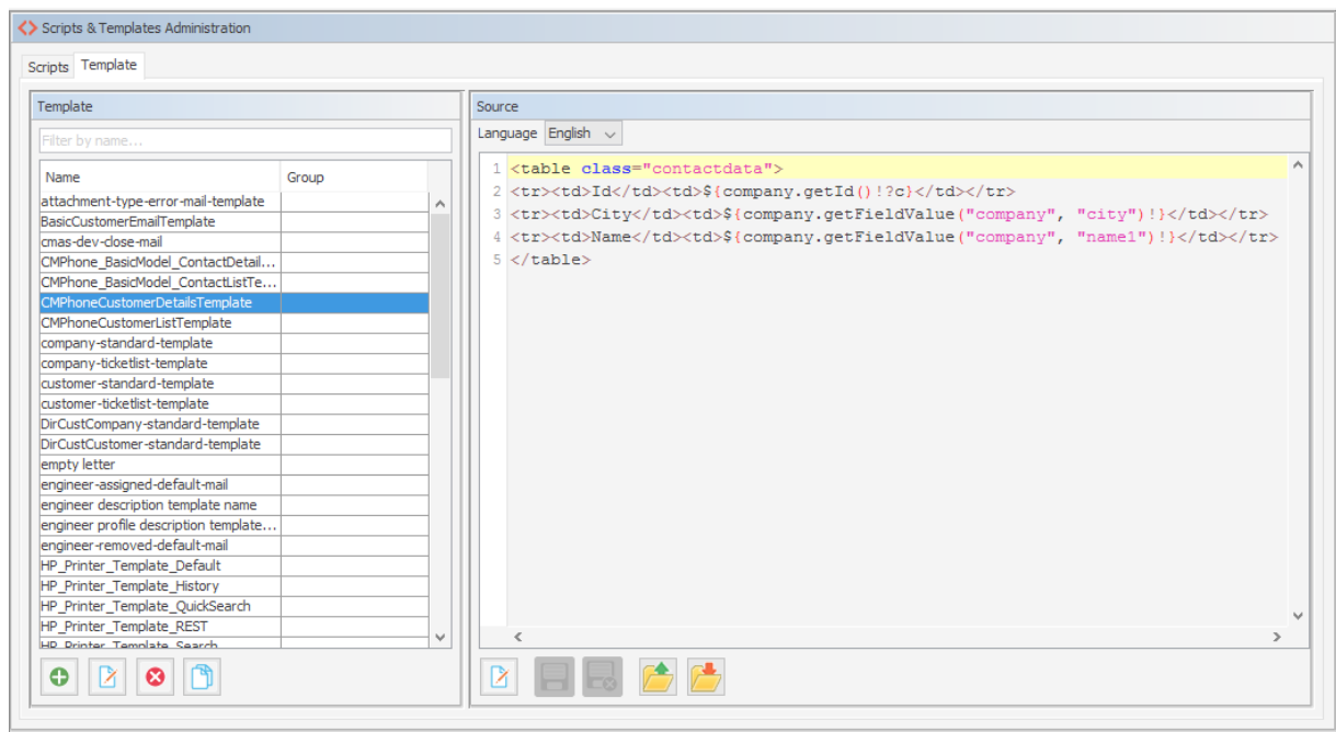
Figure 558: ConSol CM Admin Tool - System, Scripts and Templates: Example template for rendering customer data for display in CM/Phone
