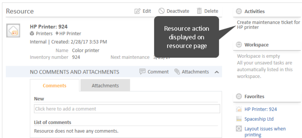
Figure 469: ConSol CM Web Client - Resource activity (based on resource action)
