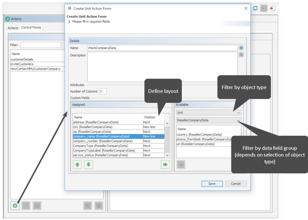
Figure 383: ConSol CM Admin Tool - Customers, Actions: Creating a new Control Form for a customer action
