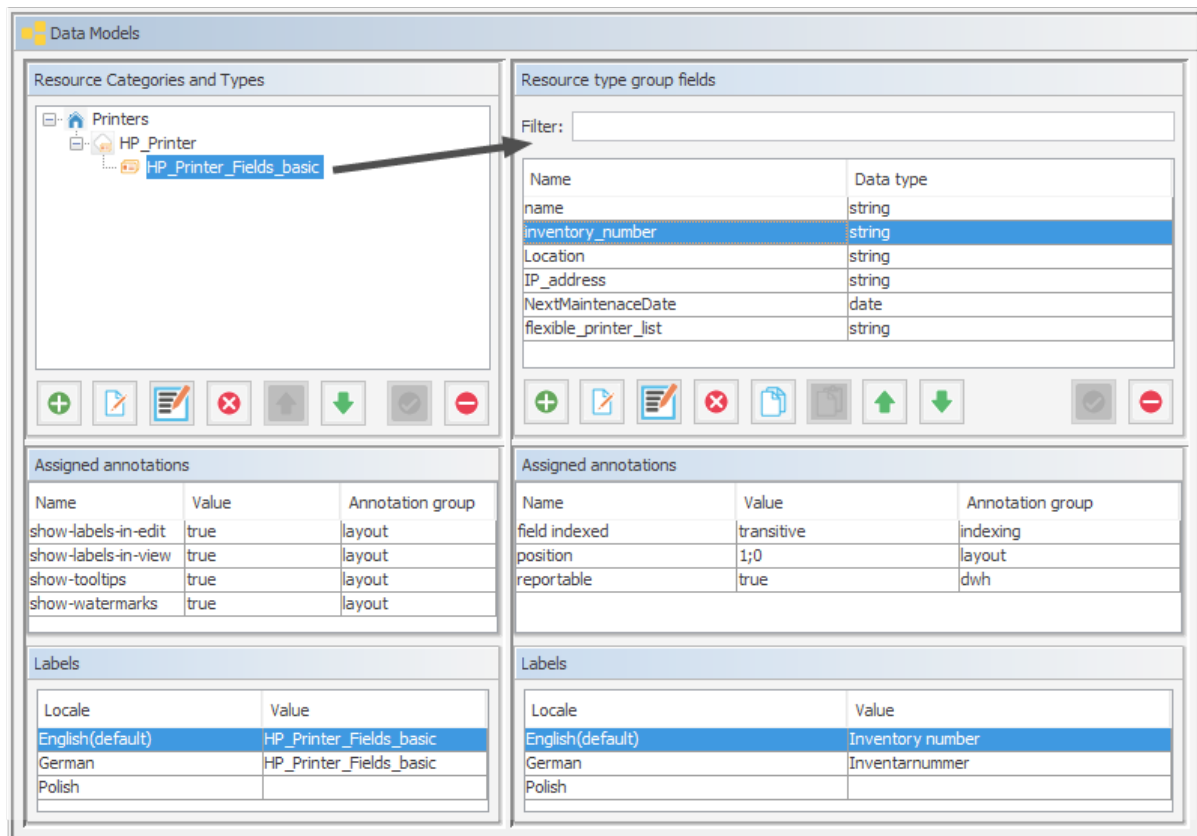
Figure 484: ConSol CM Admin Tool - Resources, Data Models: Managing resource fields
