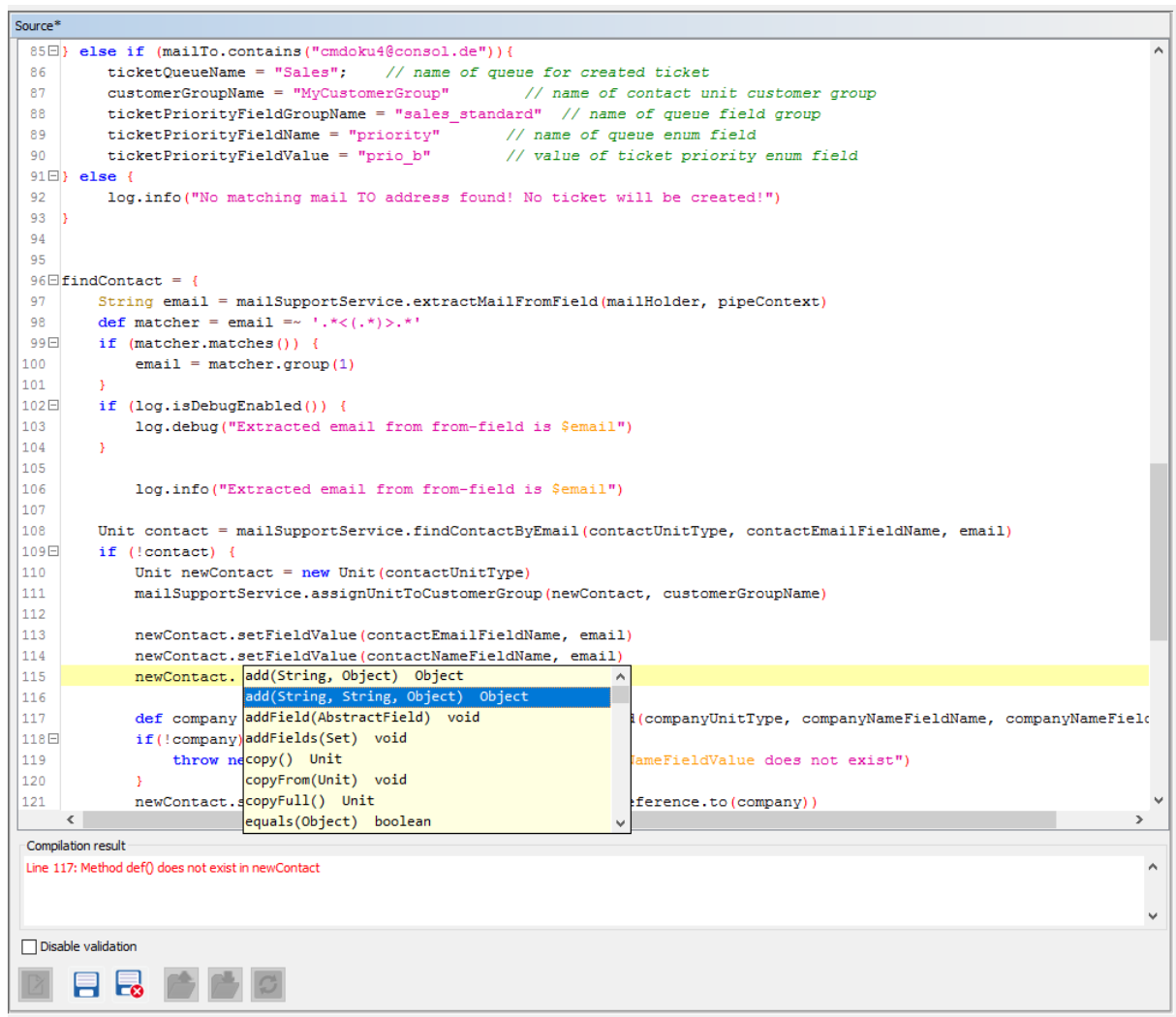
Figure 398: ConSol CM Admin Tool - System, Scripts and Templates: Source Code Editor
