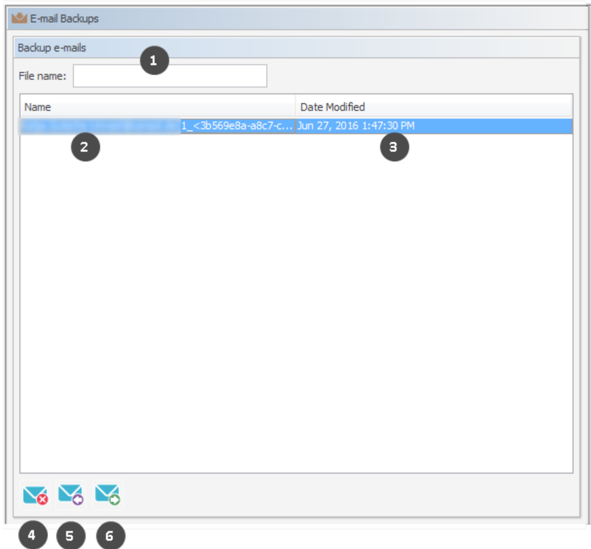
Figure 393: ConSol CM Admin Tool - Email, Email Backups
