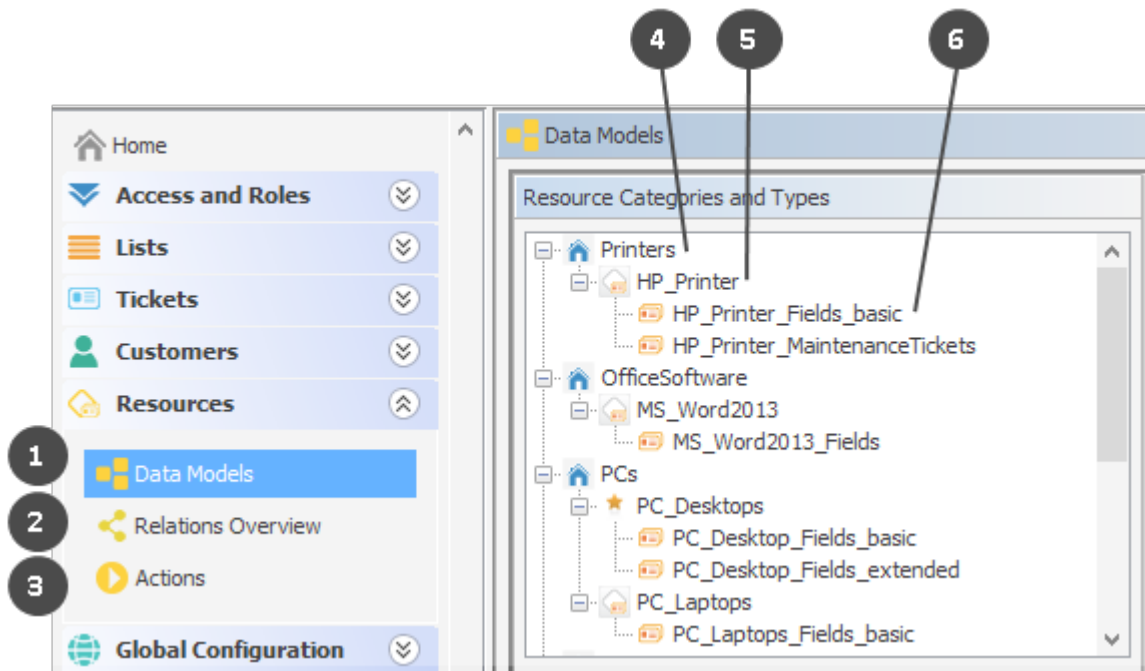
Figure 454: ConSol CM Admin Tool - Resources, Data Models: Main elements for the configuration of CM/Resource Pool
