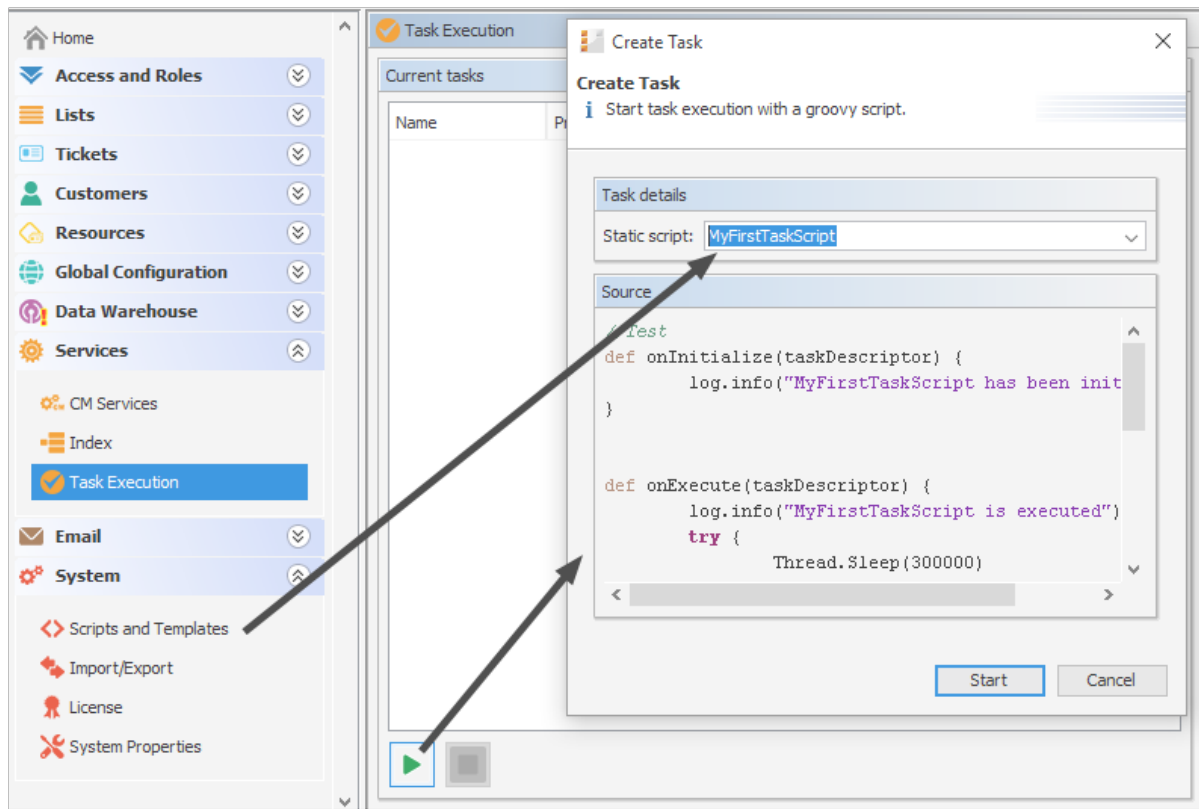
Figure 375: ConSol CM Admin Tool - Services, Task Execution: Creating a task
