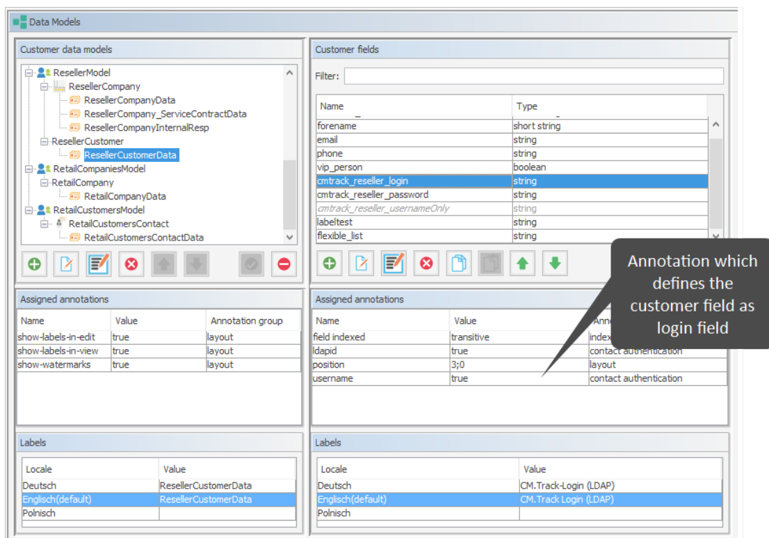
Figure 530: ConSol CM Admin Tool - Customers, Data Models: CM/Track - Annotation 'username' for login
