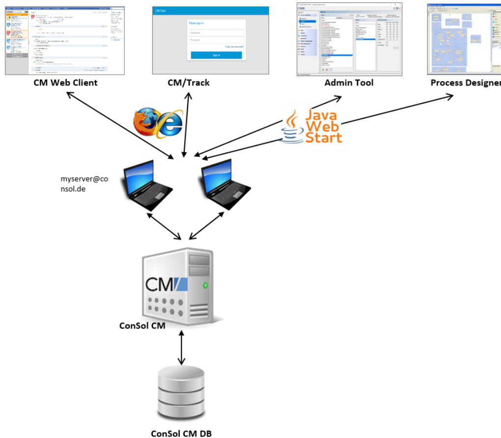
Figure 445: ConSol CM - Basic system architecture
