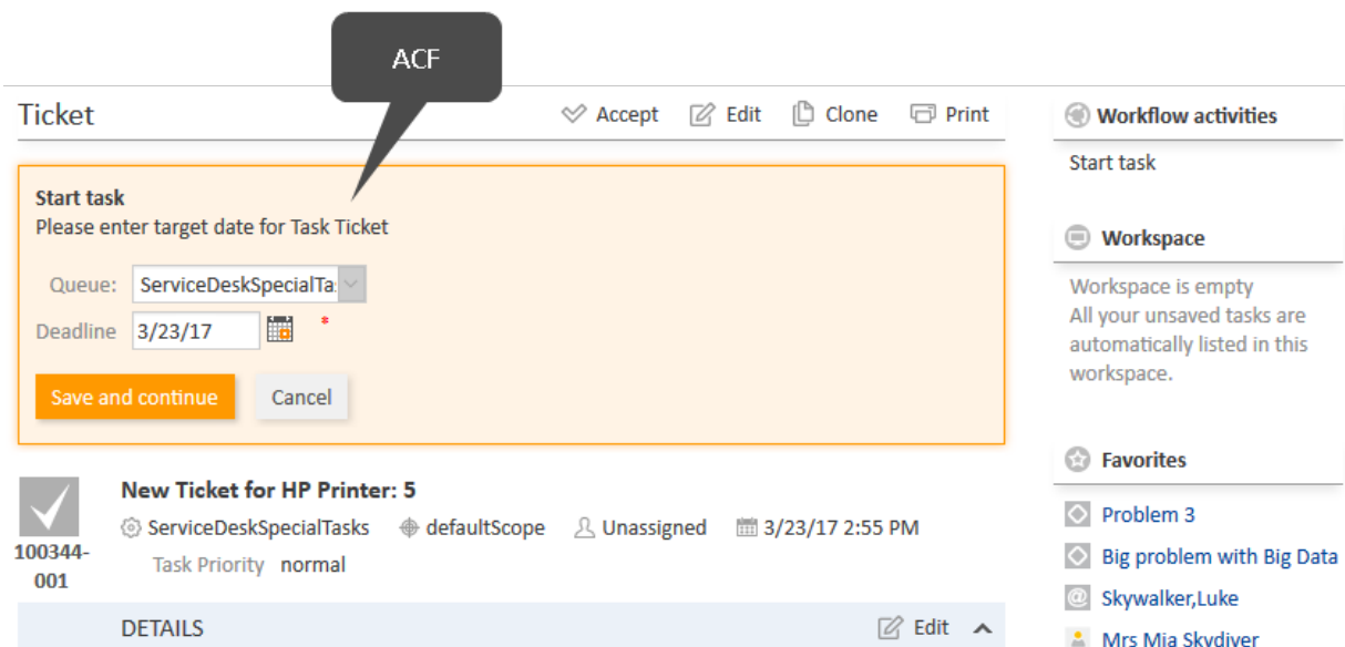
Figure 514: ConSol CM Web Client - New maintenance ticket for resource (HP Printer), ACF
