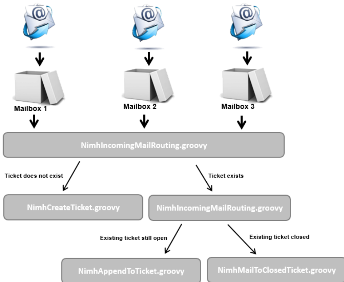
Figure 405: Email scripts (NIMH) in ConSol CM
