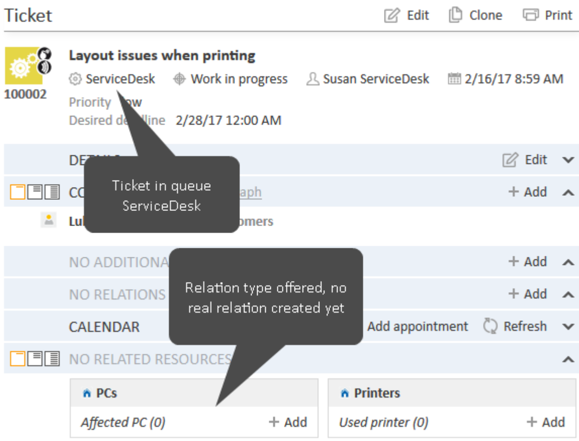
Figure 464: ConSol CM Web Client - Ticket where a relation to a PC can be created
