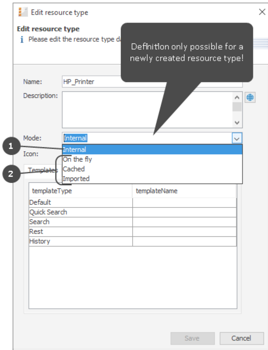
Figure 481: ConSol CM Admin Tool - Resources, Data Models: Configuration of resource type mode
