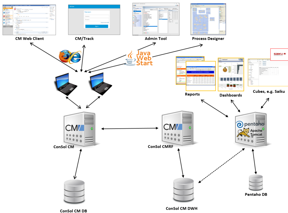
Figure 448: ConSol CM - Reporting infrastructure (2 servers)
