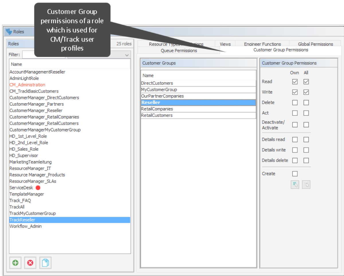
Figure 528: ConSol CM Admin Tool - Access and Roles, Roles: User profile for CM/Track, customer group permissions
