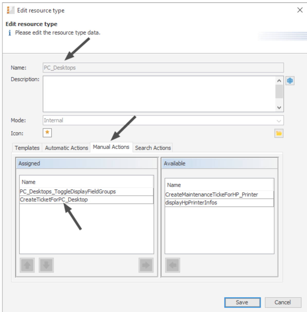
Figure 507: ConSol CM Admin Tool - Resources, Data Models: Assign the resource action to the correct resource type
