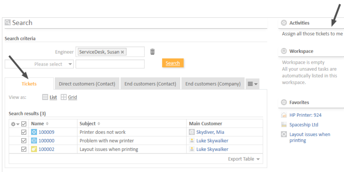
Figure 358: ConSol CM Web Client - Search actions for tickets
