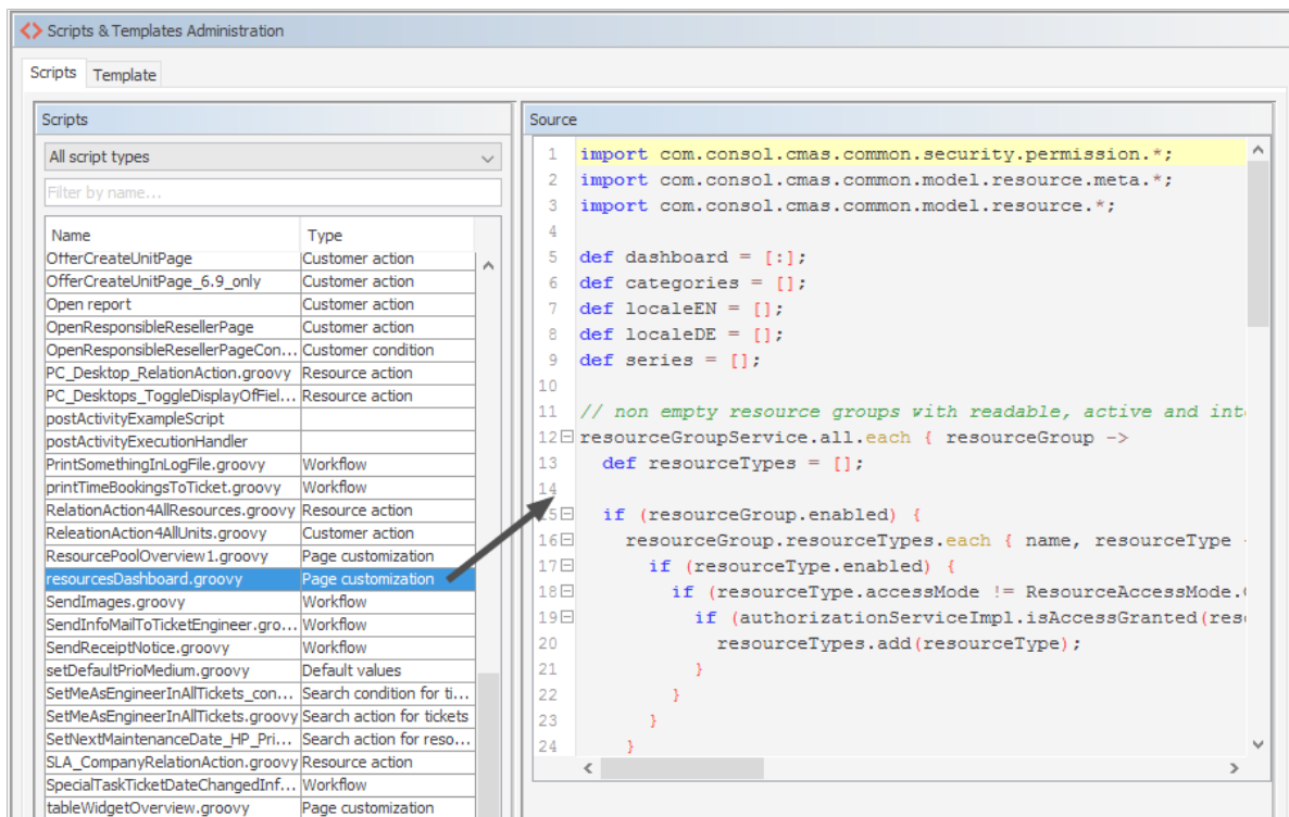
Figure 521: ConSol CM Admin Tool - System, Scripts and Templates: Admin Tool script for a widget of the Resource Pool Dashboard
