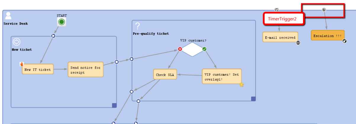
Figure 67: ConSol CM Process Designer - TimerTrigger in ServiceDesk workflow
