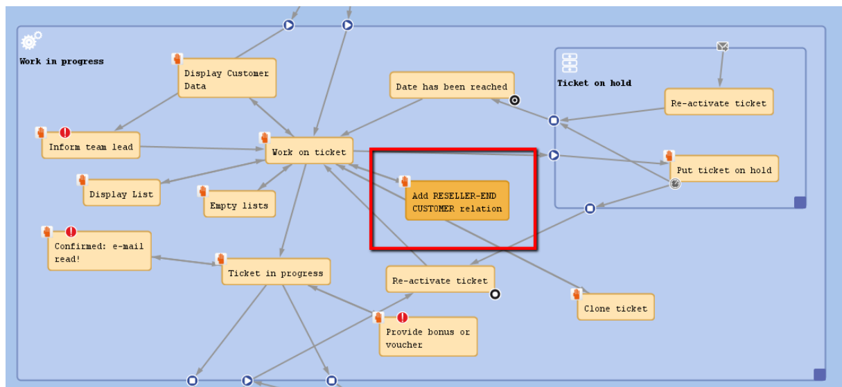
Figure 153: ConSol CM Process Designer - Workflow activity for adding a unit relation
