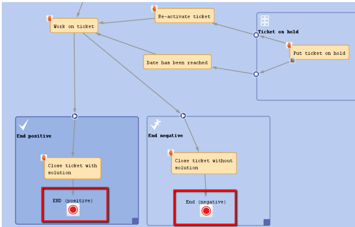
Figure 32: ConSol CM Process Designer - End nodes
