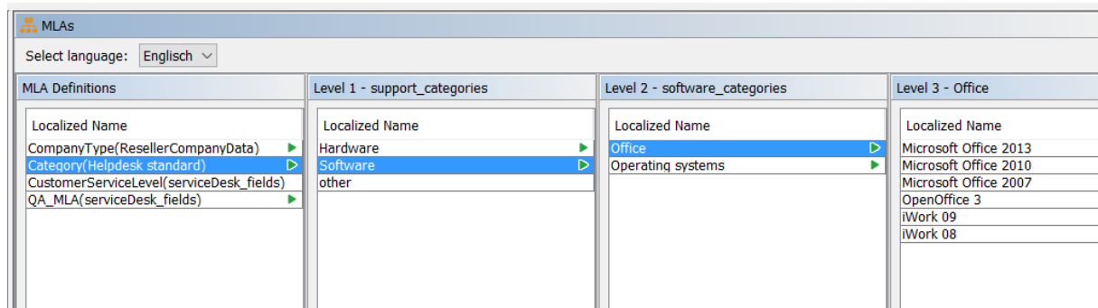
Figure 127: ConSol CM Admin Tool - MLA definition
