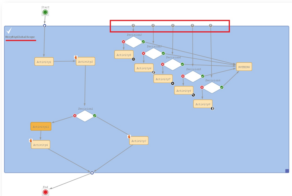
Figure 176: ConSol CM Process Designer - Scope with triggers
