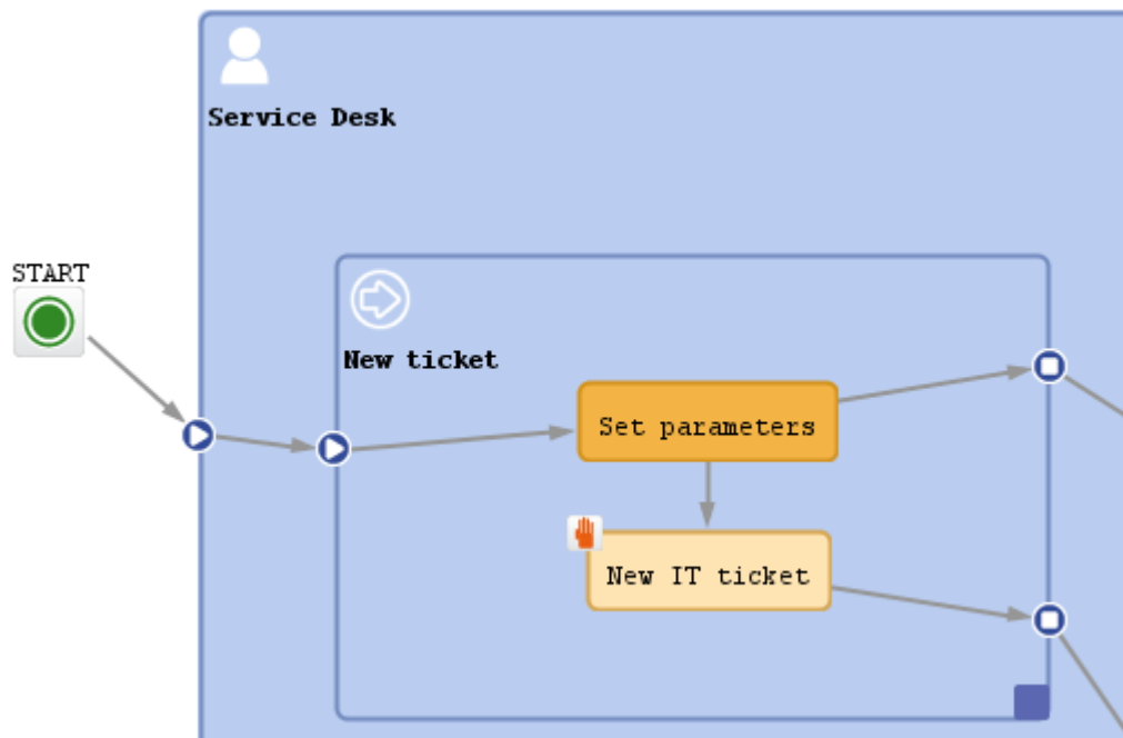
Figure 30: ConSol CM Process Designer - Start node
