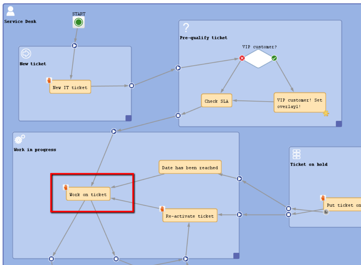
Figure 39: ConSol CM Process Designer - Manual activity in workflow
