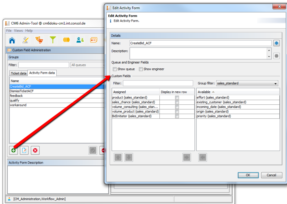
Figure 107: ConSol CM Admin Tool - ACF for Sales workflow
