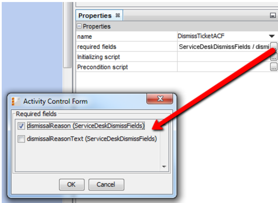
Figure 102: ConSol CM Process Designer - Properties of an ACF
