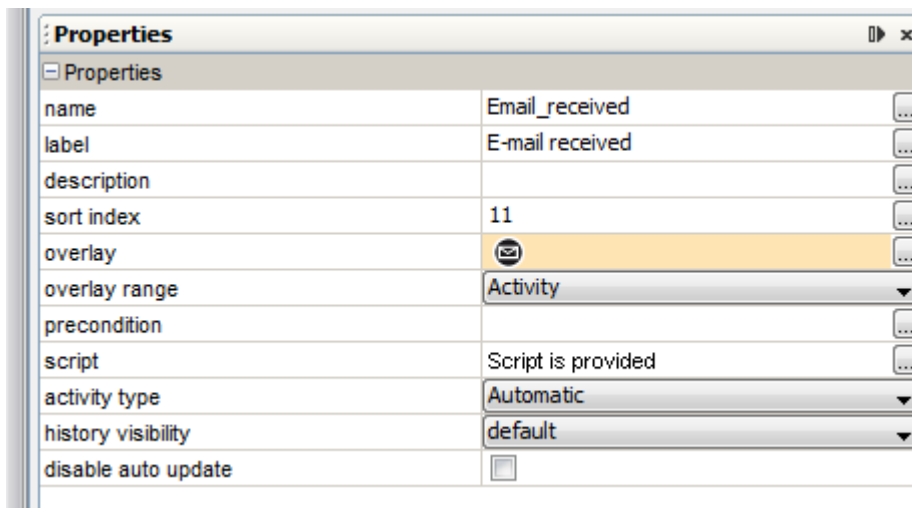
Figure 74: ConSol CM Process Designer - Use case 2: Properties of activity "E-mail received"
