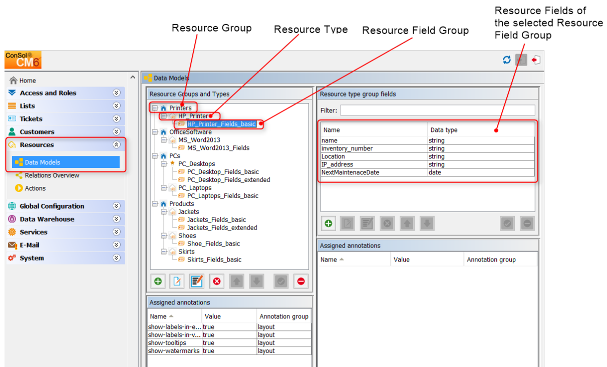
Figure 142: ConSol CM Admin Tool - Definition of the resource data model
