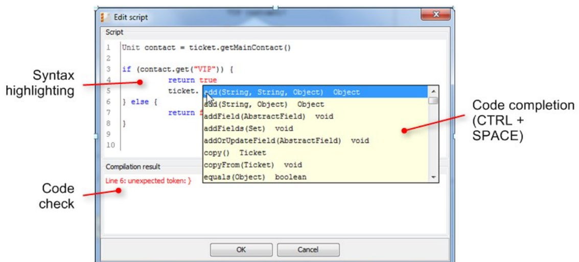
Figure 29: ConSol CM Process Designer - Script Editor
