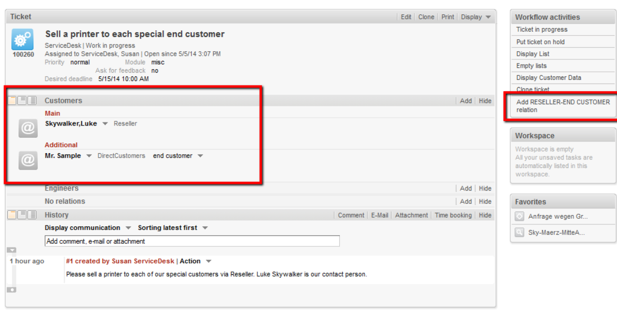
Figure 152: ConSol CM Web Client - Example ticket with main customer and one additional customer
