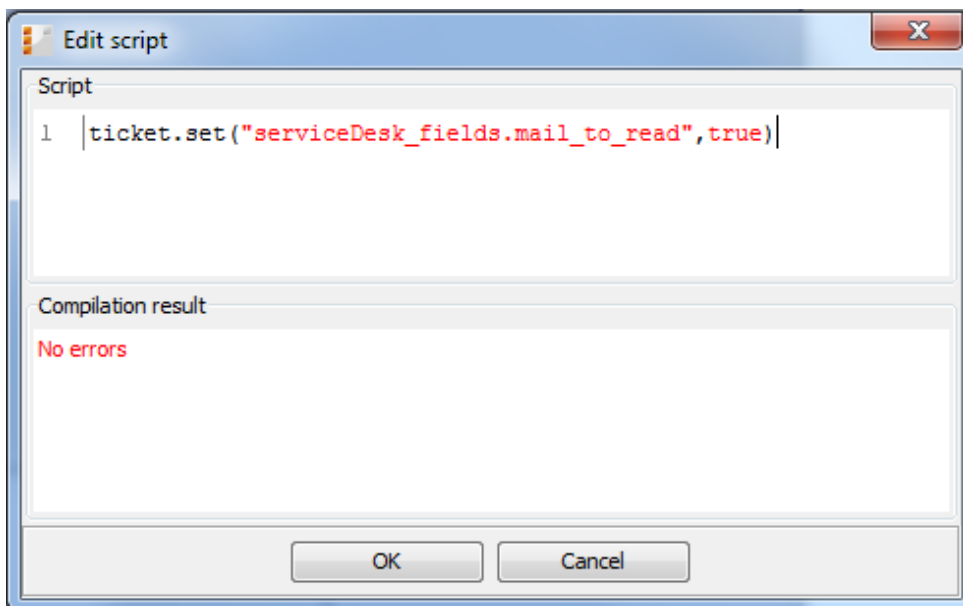
Figure 76: ConSol CM Process Designer - Use case 2: Script for activity "E-mail received"
