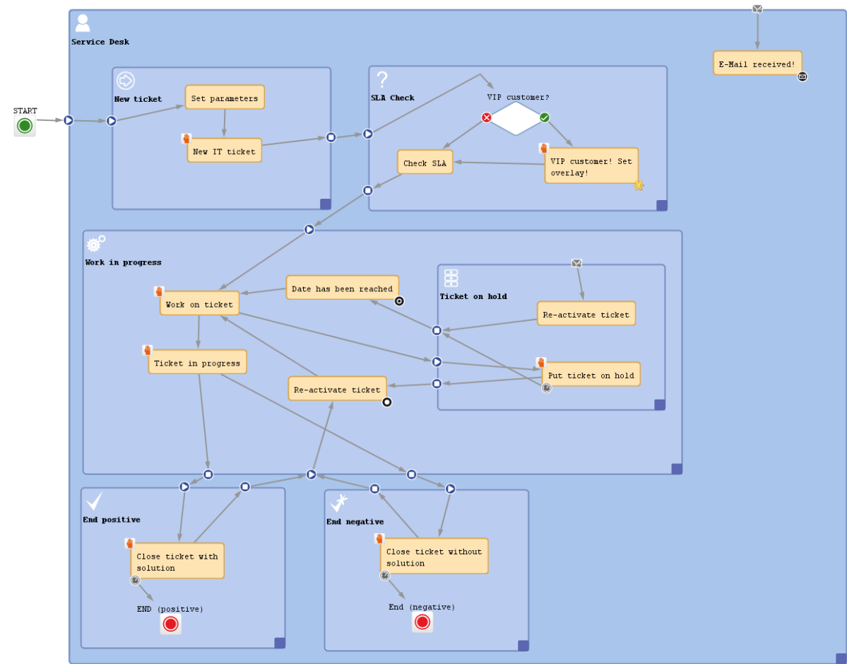
Figure 35: ConSol CM Process Designer - Workflow with scopes
