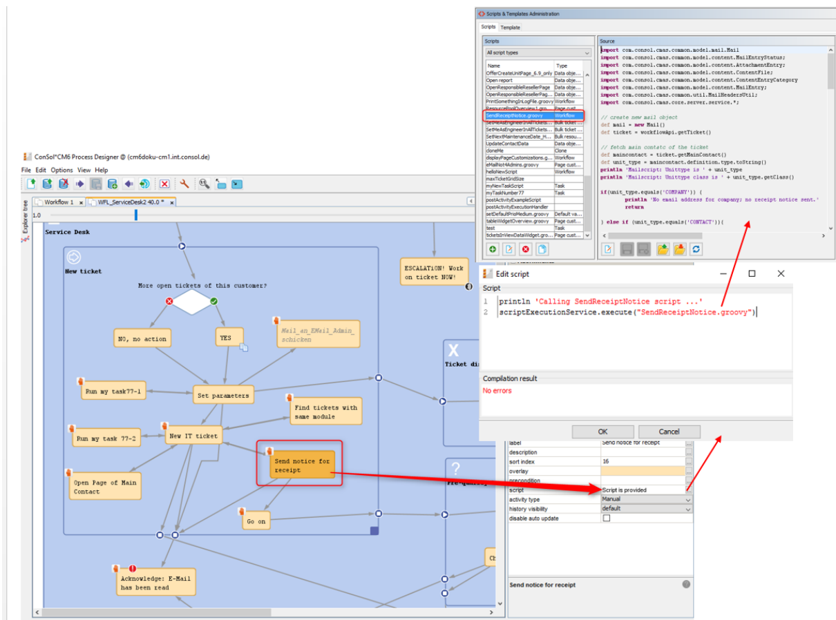
Figure 175: Calling an Admin Tool script from a workflow activity
