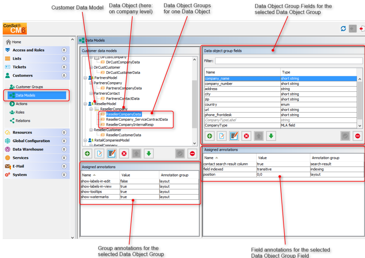
Figure 141: ConSol CM Admin Tool - Data Object Group Field administration for customer data (CM version 6.10)
