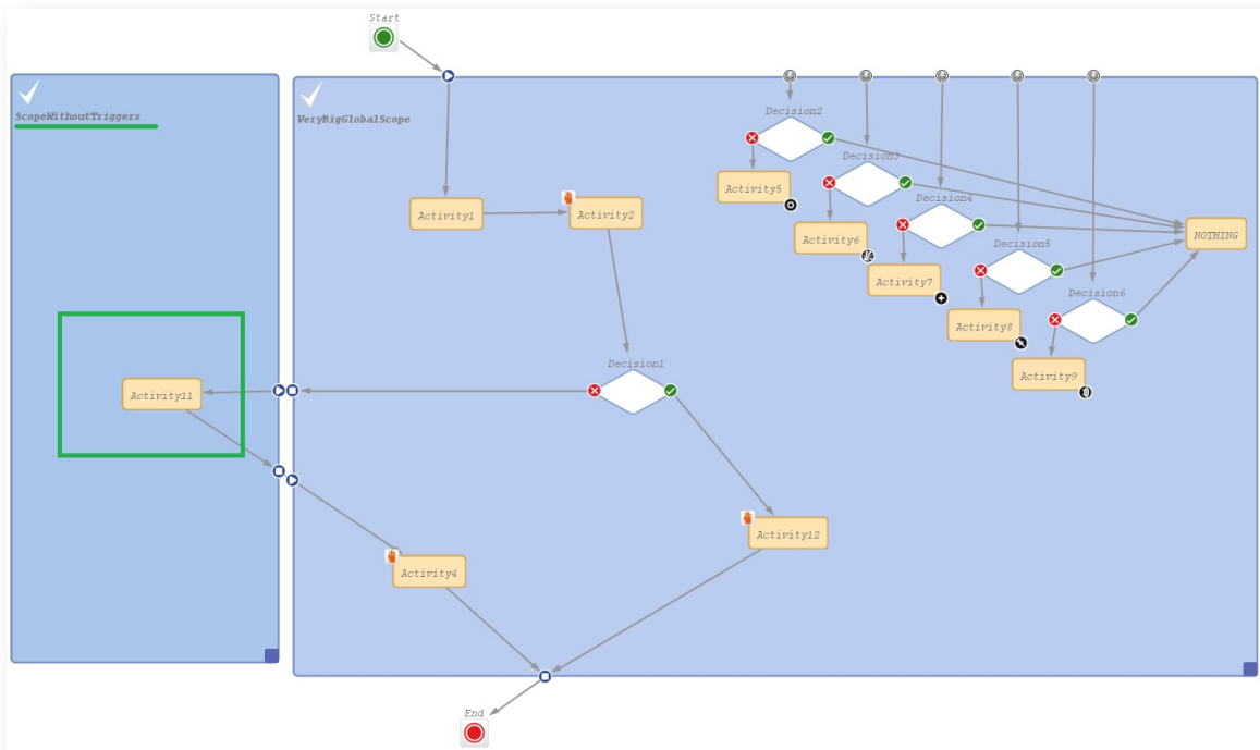
Figure 178: ConSol CM Process Designer - Separate scopes with and without triggers
