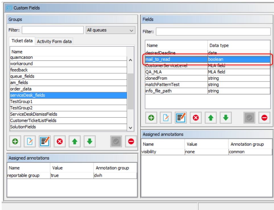
Figure 75: ConSol CM Admin Tool - Use case 2: New boolean field to register e-mail
