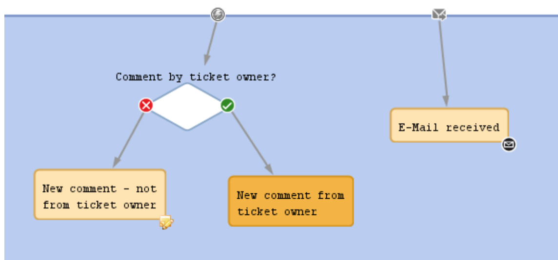
Figure 118: ConSol CM Process Designer - Two interrupts
