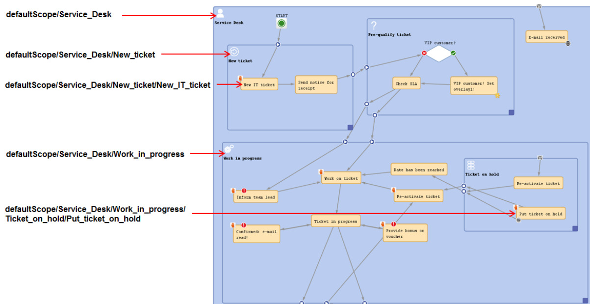
Figure 146: ConSol CM Process Designer - Path information (example: activities and scopes)
