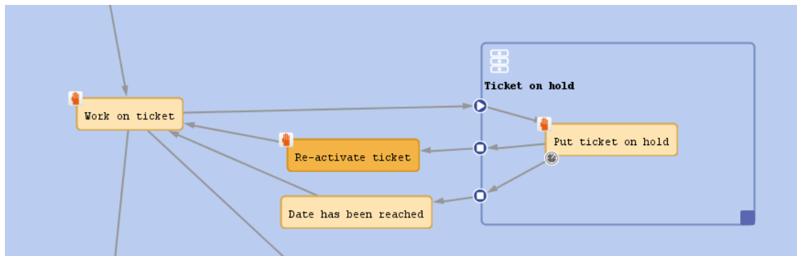
Figure 58: ConSol CM Process Designer - Use case 1: Workflow
