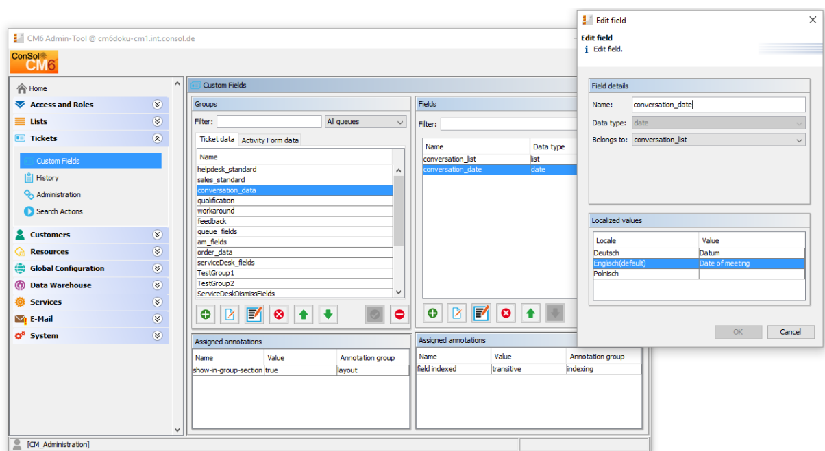
Figure 131: ConSol CM Admin Tool - Custom Fields for a list of date fields
