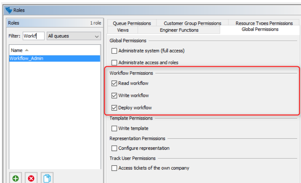
Figure 181: ConSol CM Admin Tool - Engineer permissions for deploying workflows
