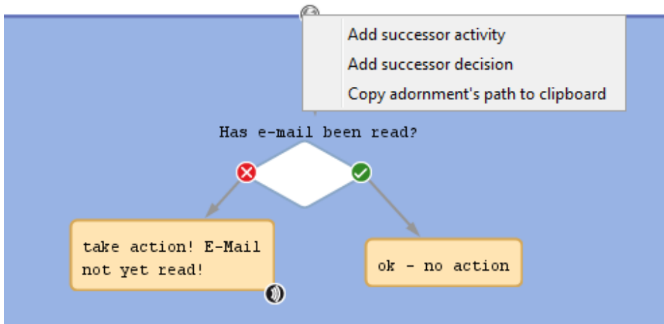
Figure 147: ConSol CM Process Designer - Copying the path of a workflow element
