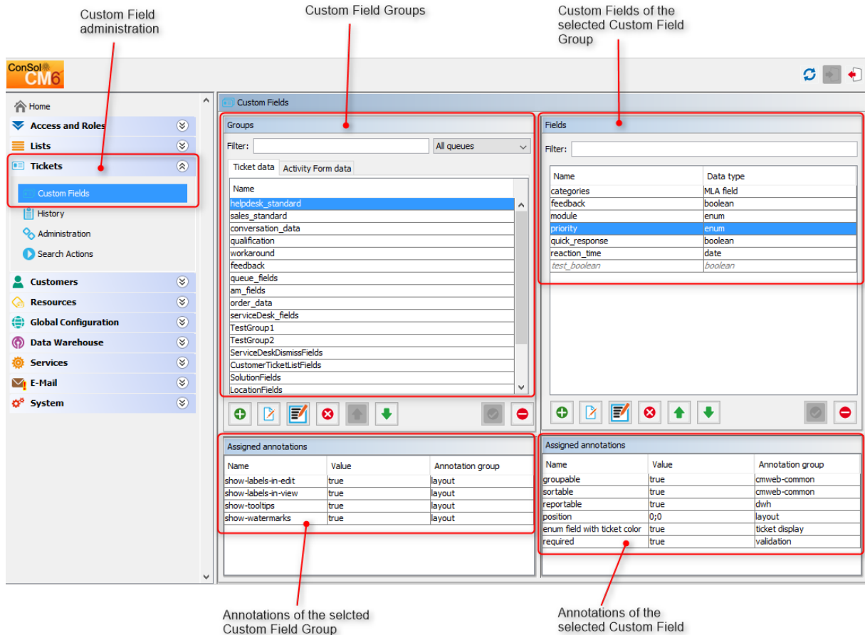
Figure 125: ConSol CM Admin Tool - Custom Field administration for ticket data (CM version 6.10)
