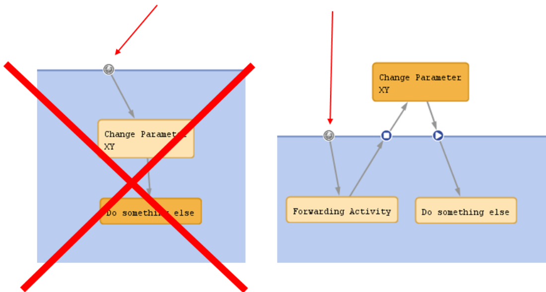
Figure 187: ConSol CM Process Designer - Avoiding self-triggering business event triggers
