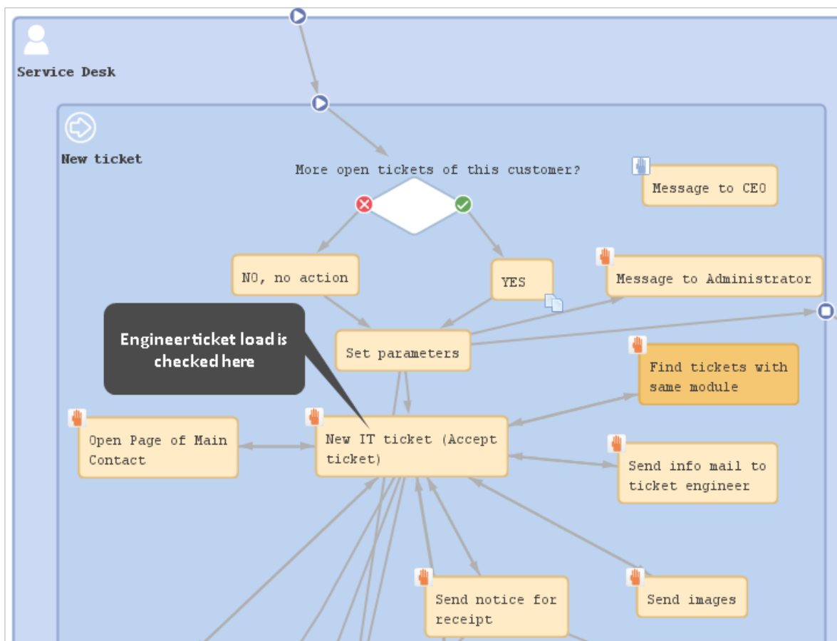
Figure 175: Workflow activity which contains the ticket number control script
