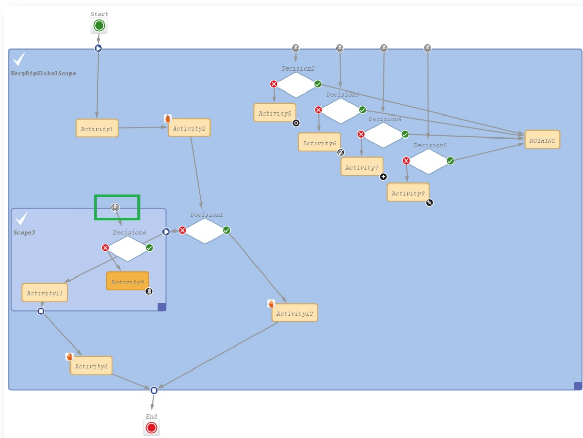
Figure 184: ConSol CM Process Designer - Move trigger to smaller scope
