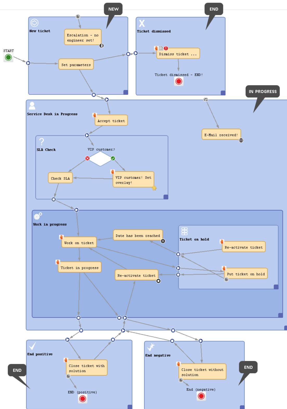
Figure 181: ConSol CM Process Designer - Workflow with three types of main scopes
