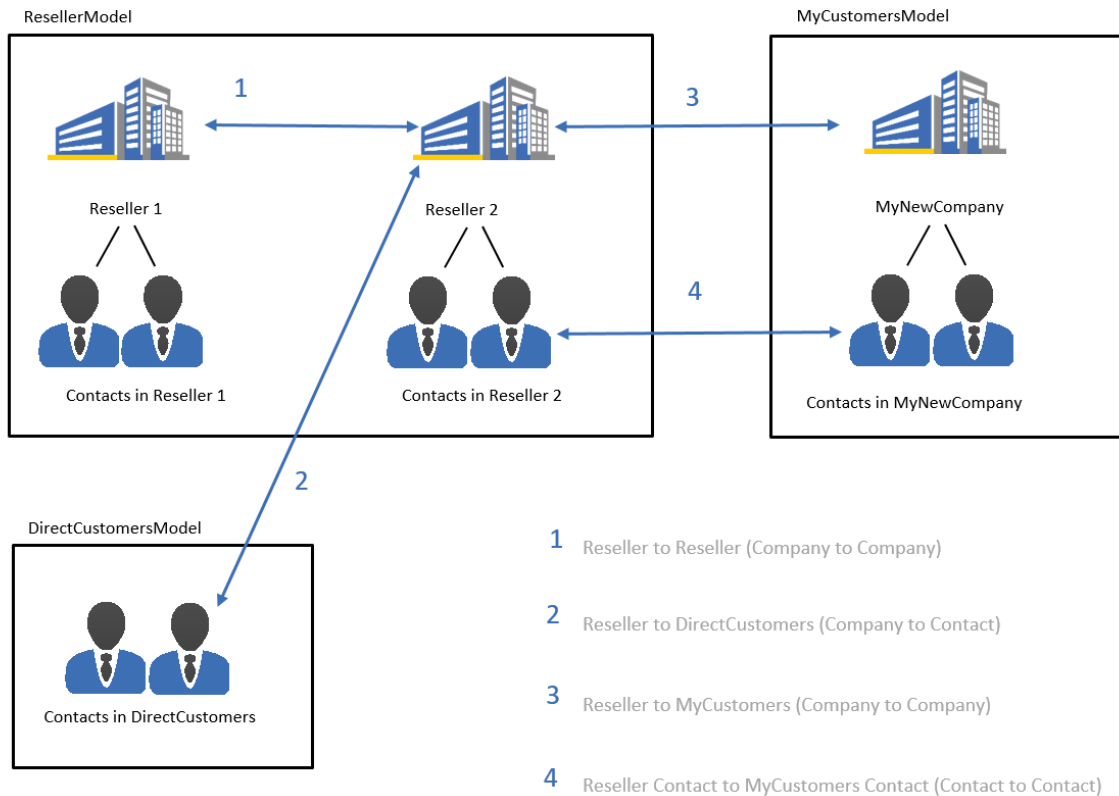
Figure 158: Customer relations in ConSol CM
