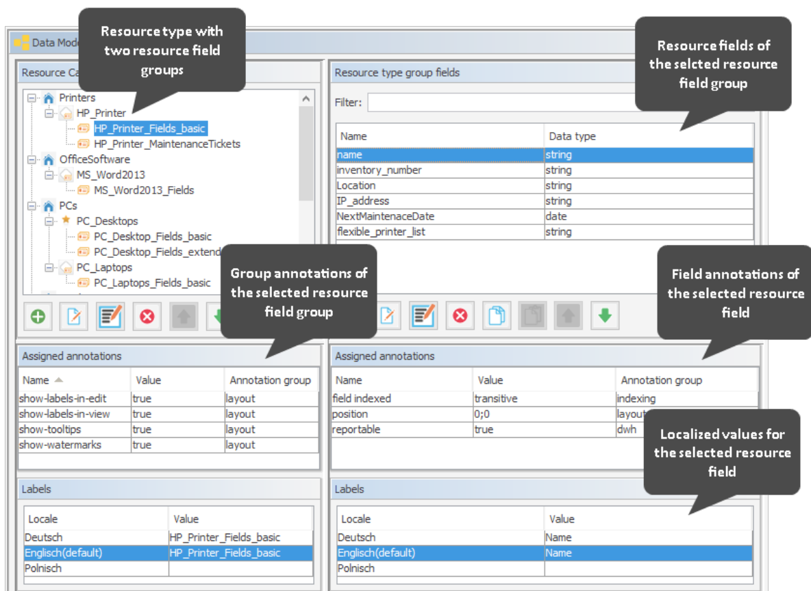
Figure 148: ConSol CM Admin Tool - Definition of the resource data model
