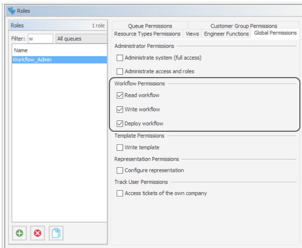
Figure 189: ConSol CM Admin Tool - Engineer permissions for deploying workflows
