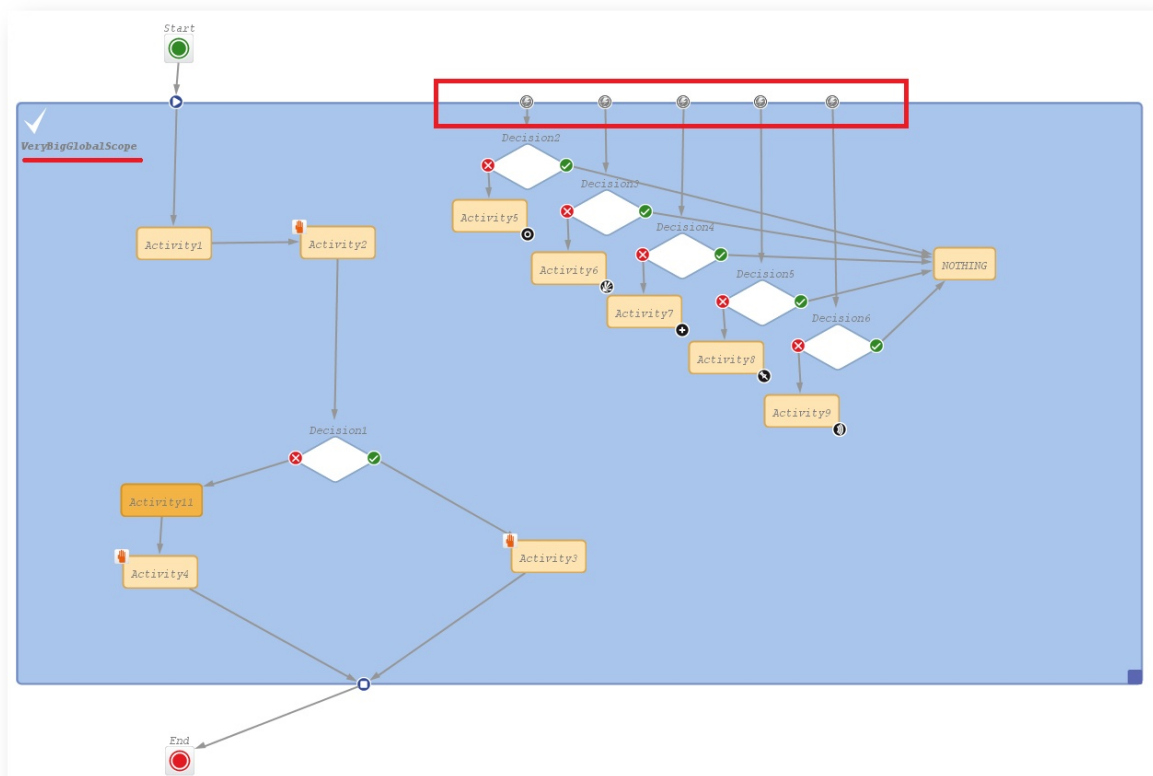
Figure 183: ConSol CM Process Designer - Scope with triggers
