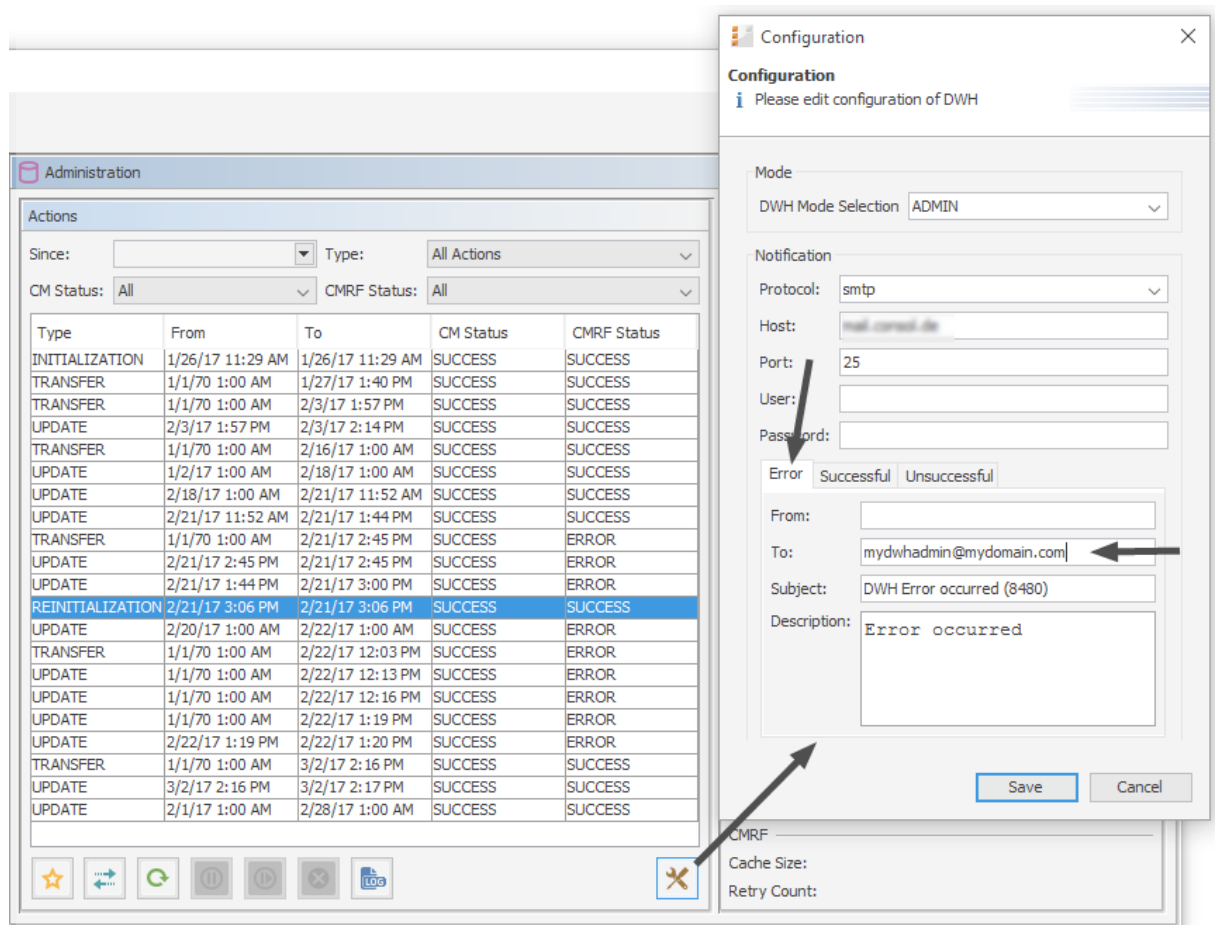
Figure 191: ConSol CM Admin Tool - Data Warehouse, Administration: Notification address for DWH errors
