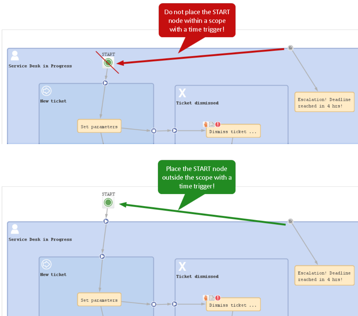
Figure 182: ConSol CM Process Designer - Position of START node
