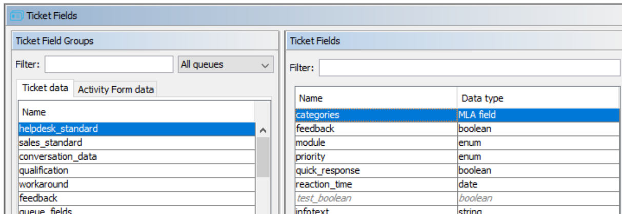
Figure 133: ConSol CM Admin Tool - Definition of a ticket field of type MLA
