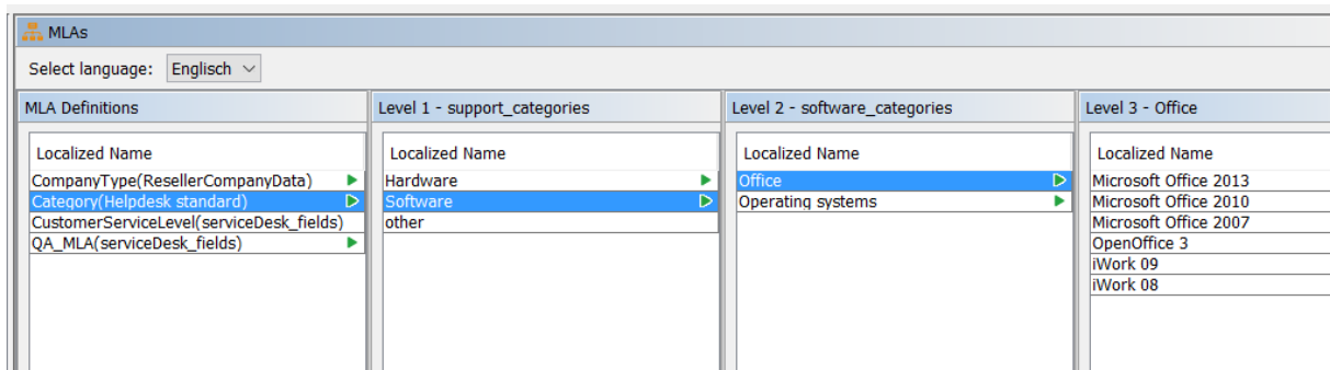
Figure 134: ConSol CM Admin Tool - MLA definition
