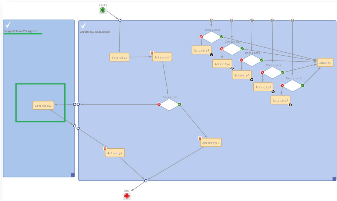
Figure 182: ConSol CM Process Designer - Separate scopes with and without triggers
