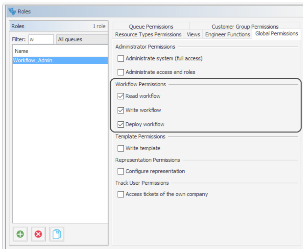
Figure 186: ConSol CM Admin Tool - Engineer permissions for deploying workflows
