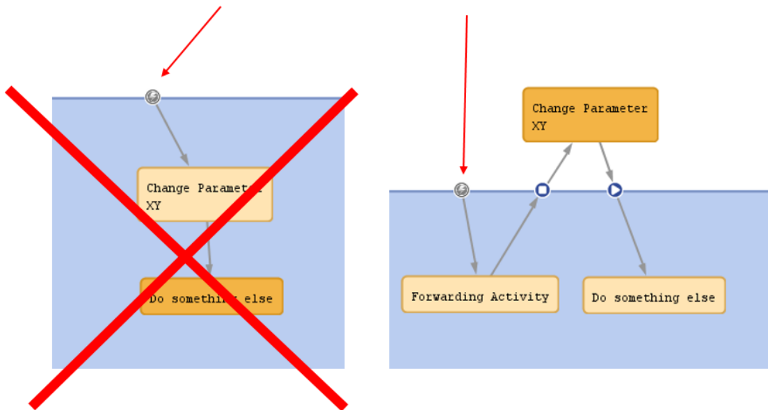
Figure 159: ConSol CM Process Designer - Avoiding self-triggering business event triggers
