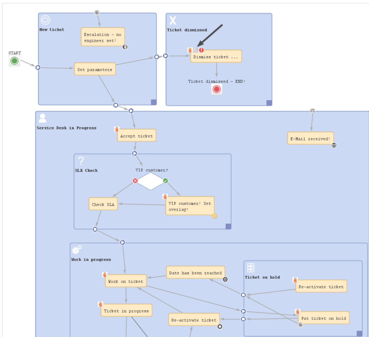
Figure 101: ConSol CM Process Designer - ACF in workflow
