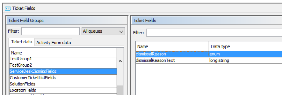
Figure 99: ConSol CM Admin Tool - definition of ticket fields which will later be used in an ACF
