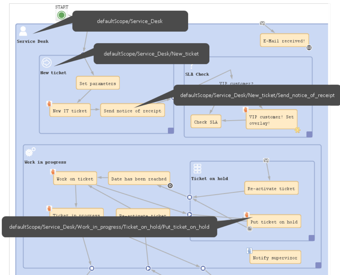
Figure 128: ConSol CM Process Designer - Path information (example: activities and scopes)
