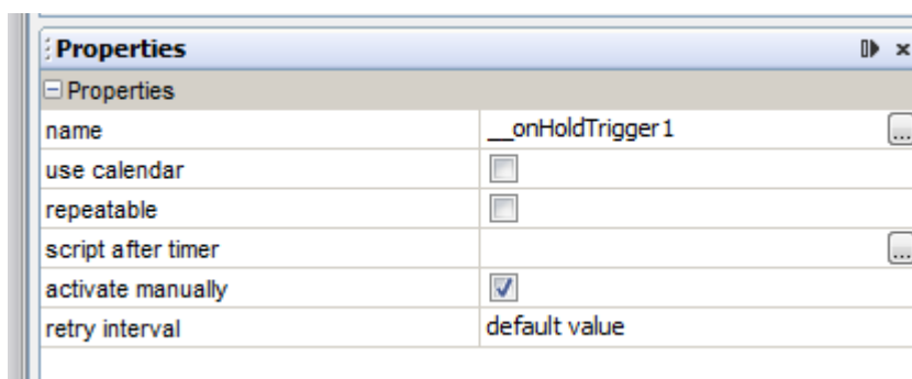
Figure 59: ConSol CM Process Designer - Use case 1: Properties editor for time trigger
