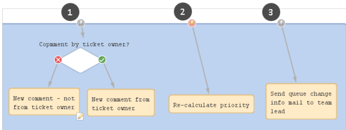
Figure 82: ConSol CM Process Designer - Firing order of business event triggers (1)
