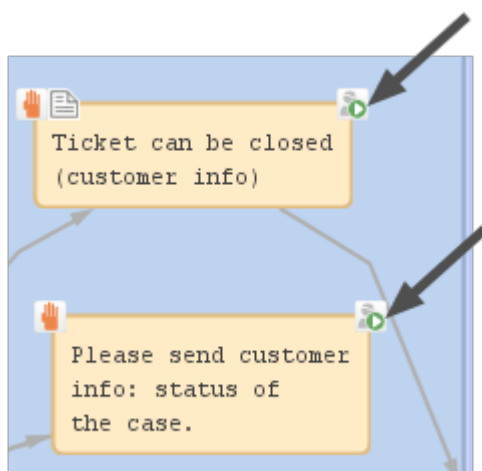
Figure 37: ConSol CM Process Designer - Two activities which should be displayed for CM/Track customers ("exposed to customers")
