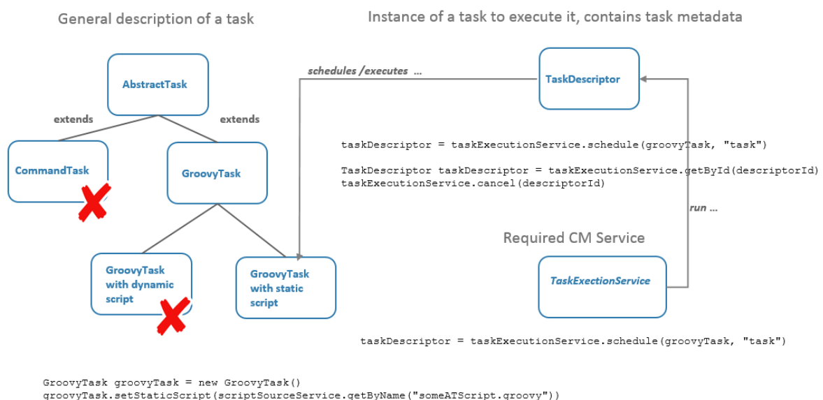
Figure 407: Some TEF Groovy classes
