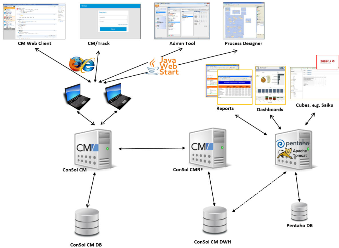
Figure 543: ConSol CM - Reporting infrastructure (2 servers)
