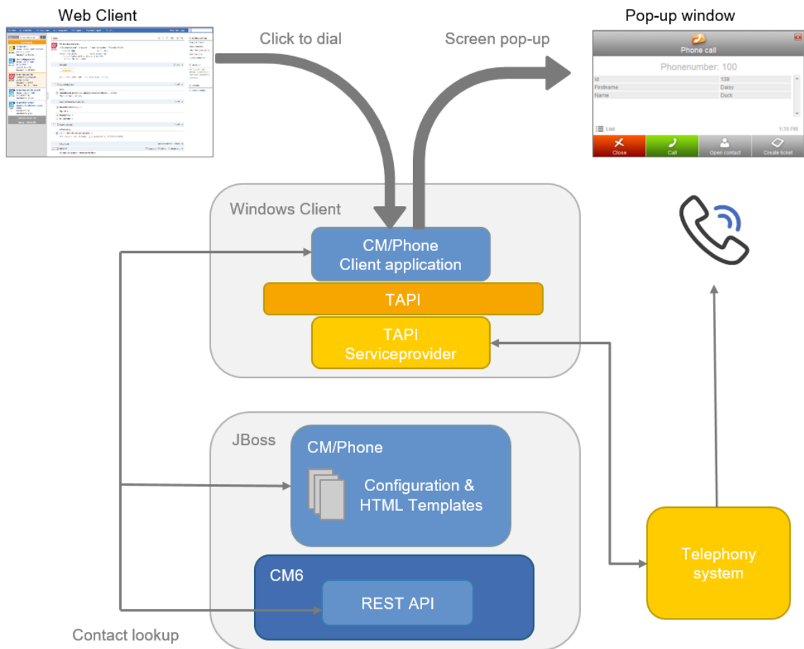
Figure 665: ConSol CM/Phone - Basic principle
