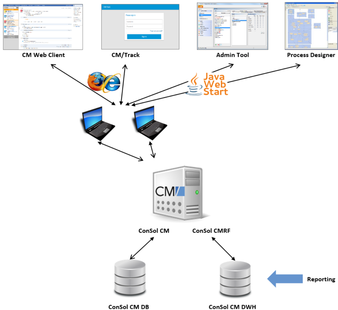
Figure 542: ConSol CM - Infrastructure with CMRF and DWH (1 server)
