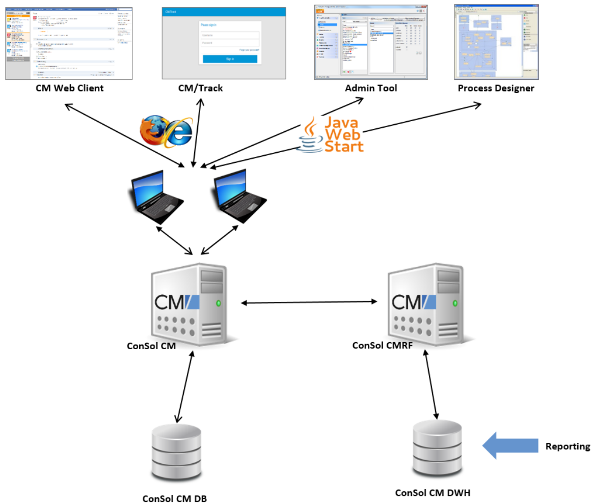
Figure 361: ConSol CM - System architecture with DWH and CMRF (2 servers)
