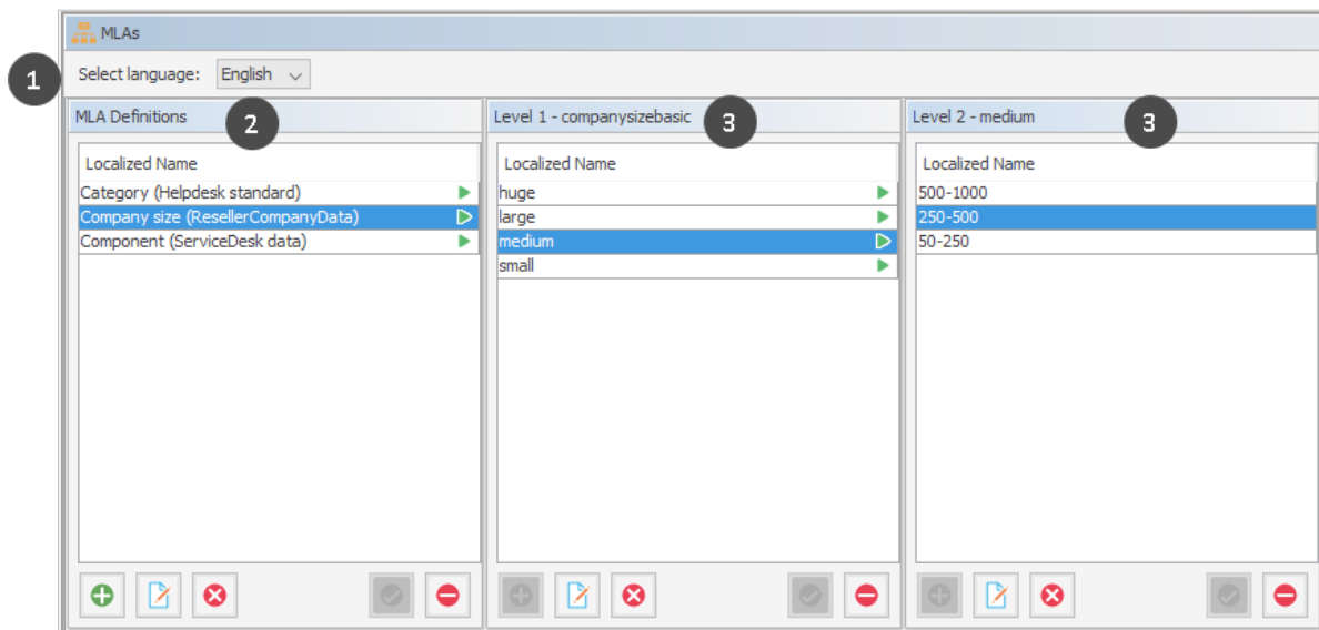
Figure 59: ConSol CM Admin Tool - Lists, MLAs
