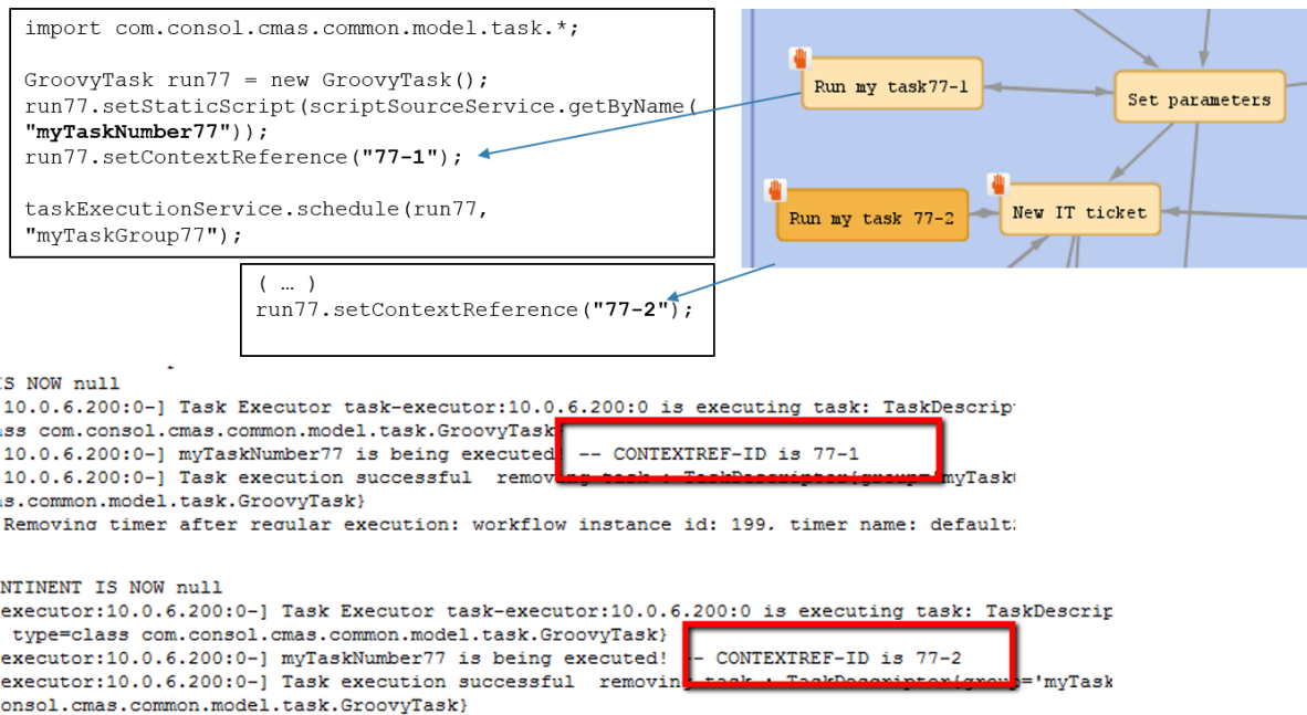
Figure 382: Workflow activities and log output when one of the activities has called the TEF script
