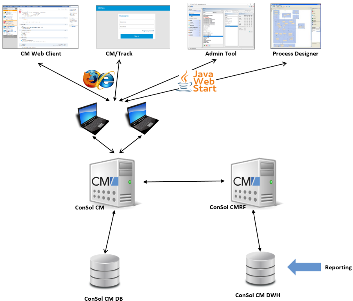
Figure 447: ConSol CM - Infrastructure with CMRF and DWH (2 servers)
