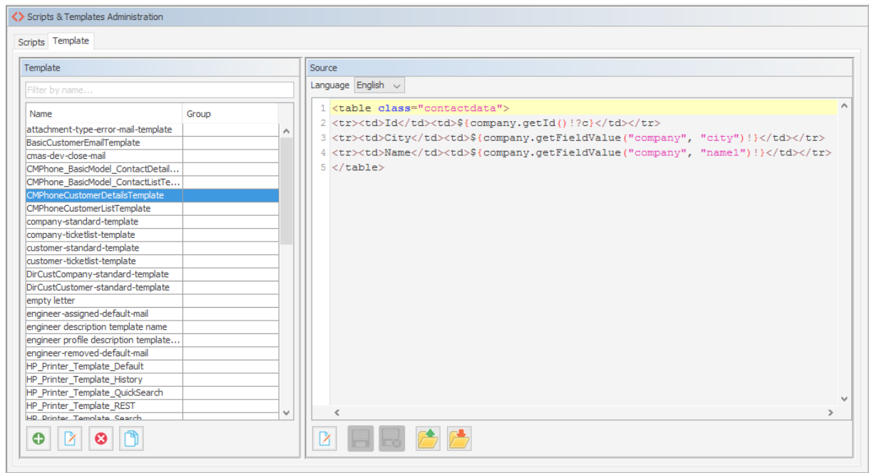
Figure 557: ConSol CM Admin Tool - System, Scripts and Templates: Example template for rendering customer data for display in CM/Phone
