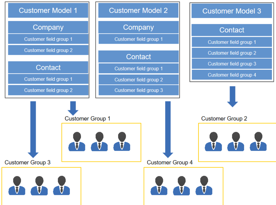
Figure 88: ConSol CM customer data models - General principle
