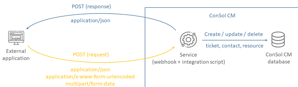
Figure 445: Webhooks in ConSol CM
