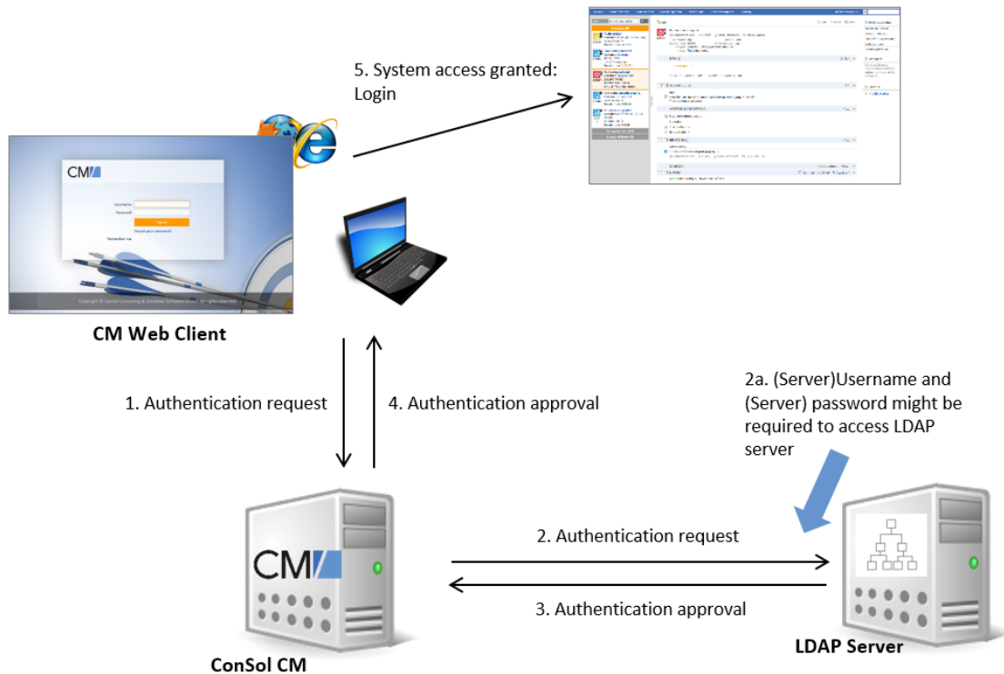
Figure 440: ConSol CM - LDAP authentication process
