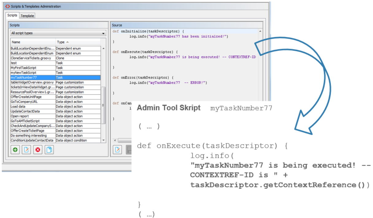
Figure 381: ConSol CM Admin Tool - System, Scripts and Templates: Admin Tool script for a TEF task
