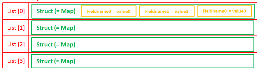
Figure 43: List of structs, technical principle
