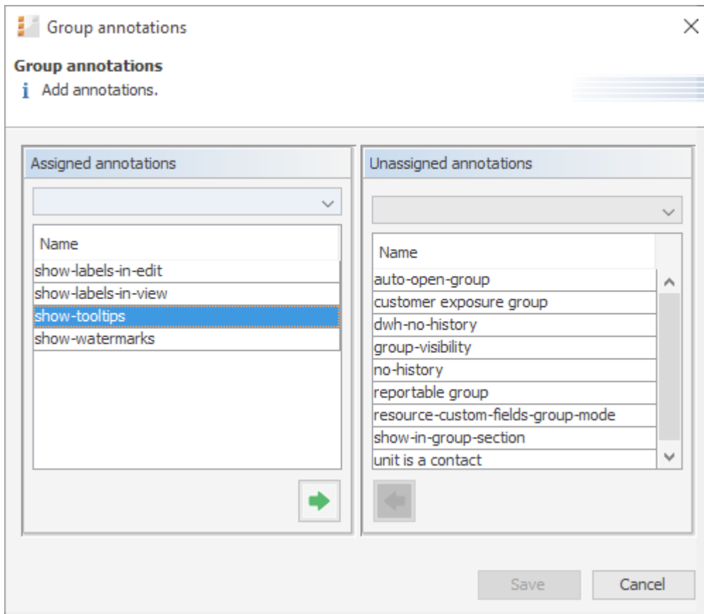
Figure 484: ConSol CM Admin Tool - Resources, Data Models: Resource field group annotations
