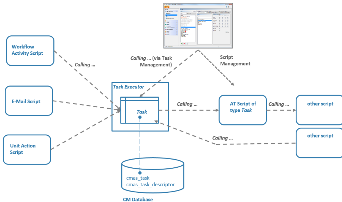
Figure 375: ConSol CM Task Execution Framework
