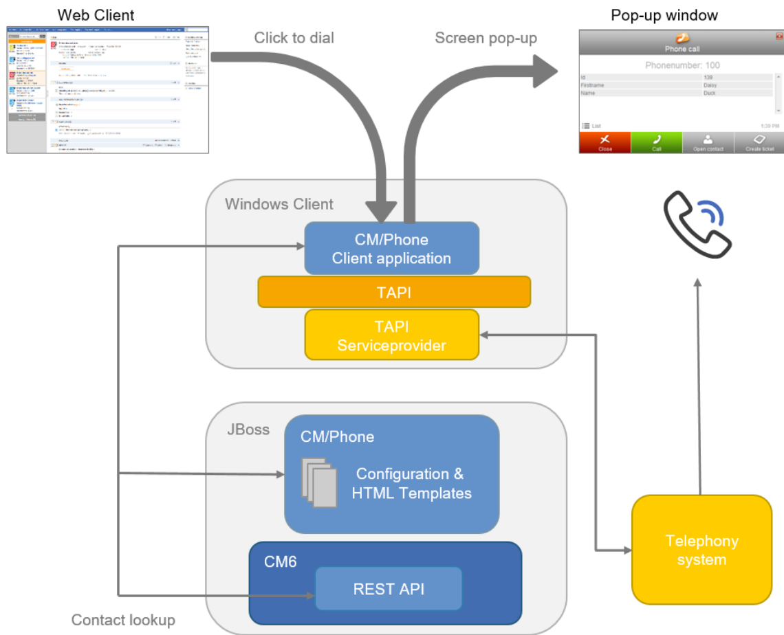
Figure 554: ConSol CM/Phone - Basic principle
