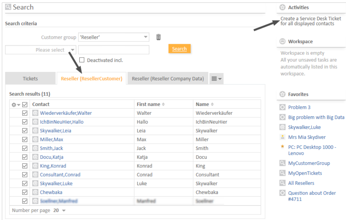
Figure 368: ConSol CM Web Client - Search action on customers (here: contacts), 1
