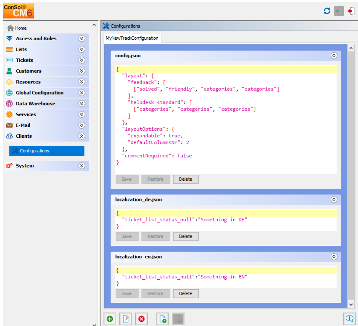
Figure 325: ConSol CM Admin Tool - REST client configuration (example)
