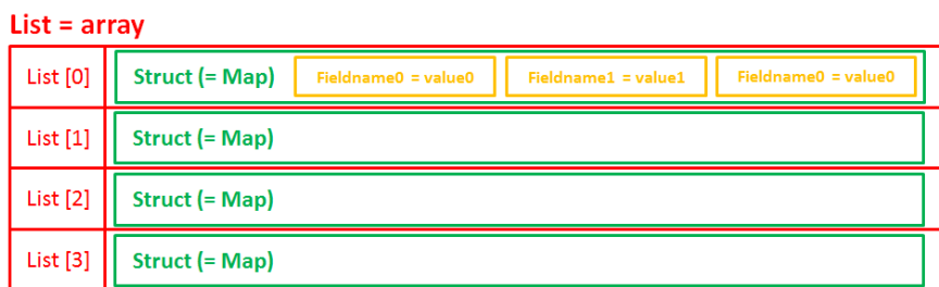
Figure 117: List of structs, technical principle
