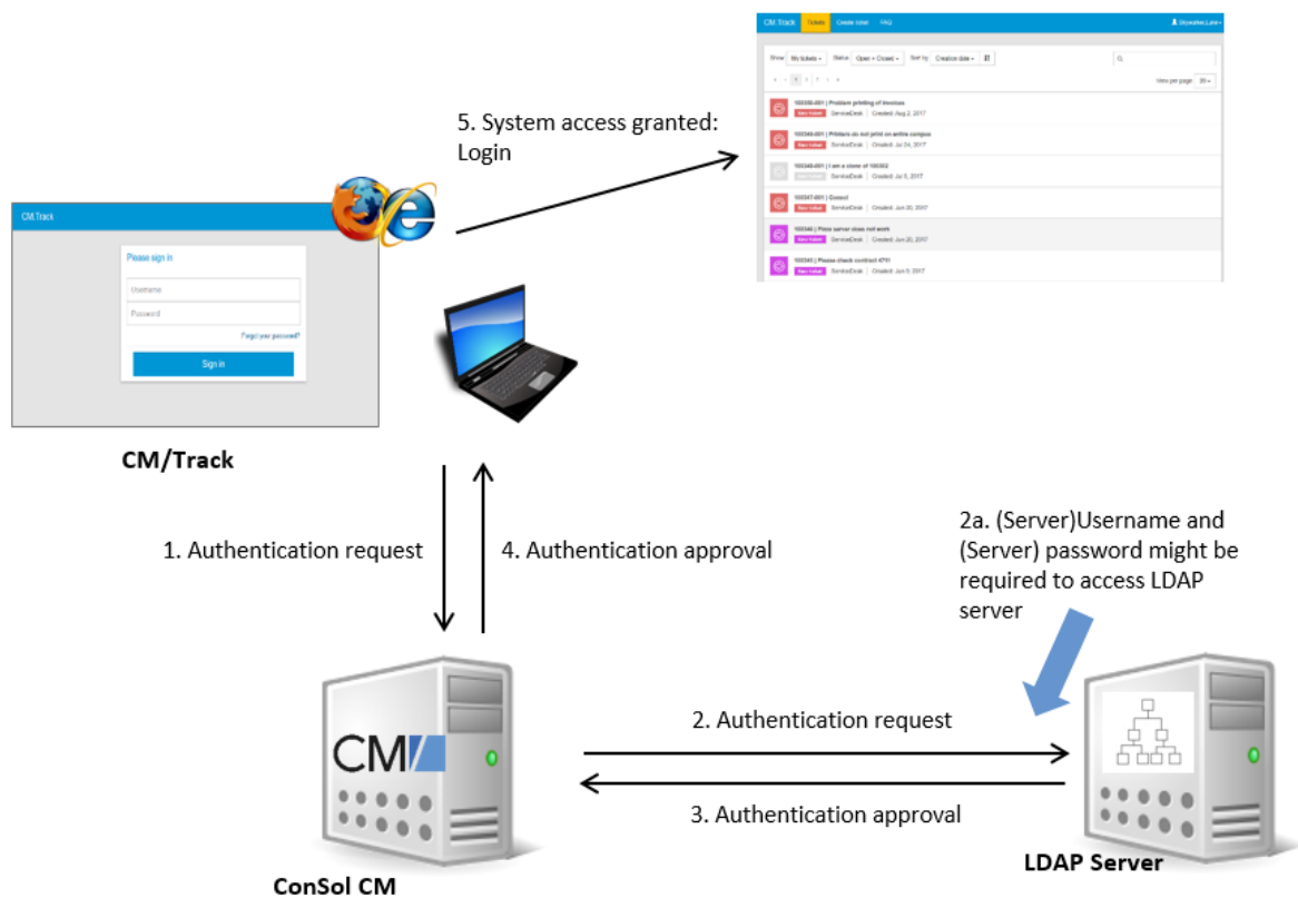
Figure 526: ConSol CM - LDAP authentication process for CM/Track
