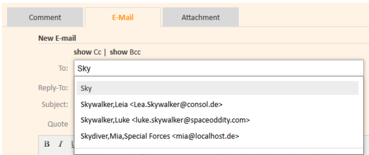
Figure 353: ConSol CM Web Client - Ticket Email Editor: Automatic search for contacts as email receivers
