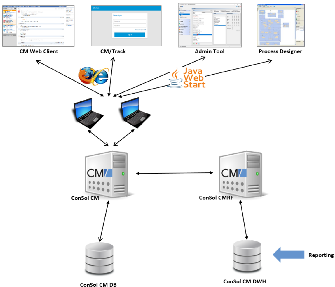
Figure 335: ConSol CM - System architecture with DWH and CMRF (2 servers)
