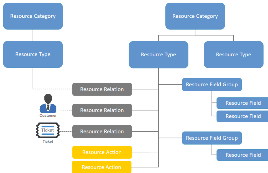
Figure 453: CM/Resource Pool - Objects in a resource model
