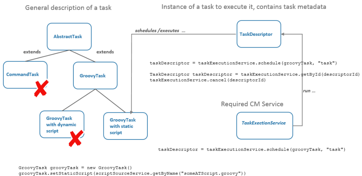
Figure 378: Some TEF Groovy classes
