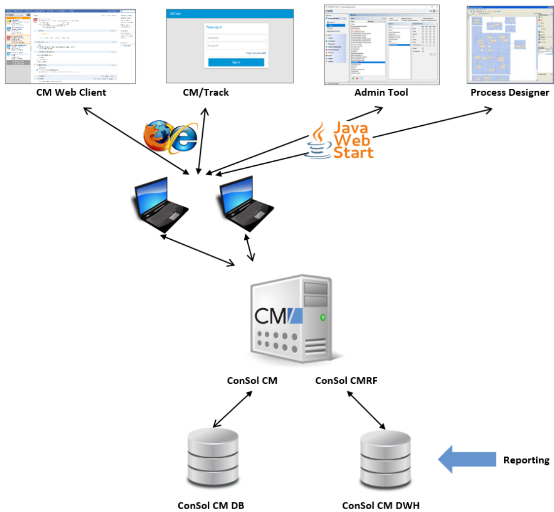
Figure 448: ConSol CM - Infrastructure with CMRF and DWH (1 server)
