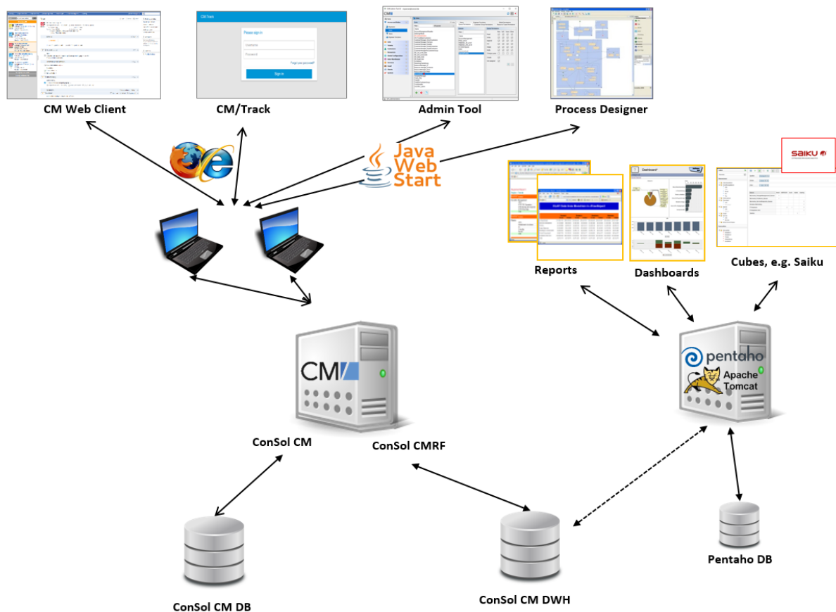
Figure 450: ConSol CM - Reporting infrastructure (1 server)
